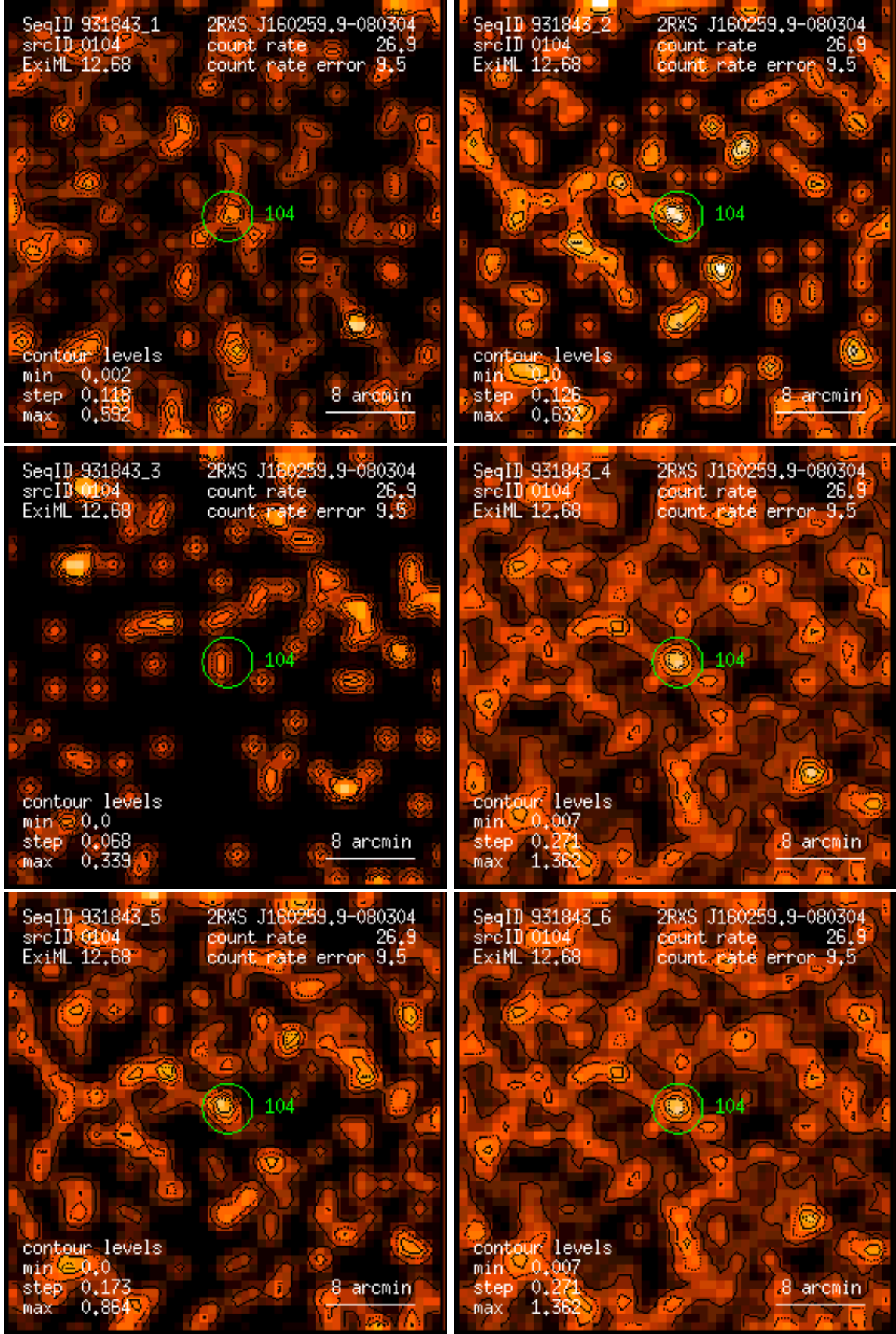
Figure 104: RASS 931843: detection 0104: band rate images, Gaussian filter: (1) PSPC channels 11 – 41, (2) 52 – 90, (3) 91 – 201, (4) 11 – 235, (5) 52 – 201, (6) 11 – 201. Broad band rates in counts/ks. Band rate contour levels in counts/ks/arcmin 2 .
