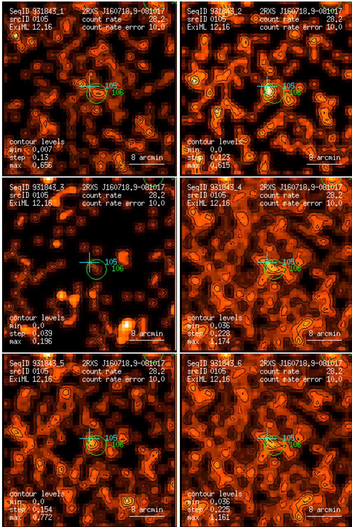
Figure 105: RASS 931843: detection 0105: band rate images, Gaussian filter: (1) PSPC channels 11 – 41, (2) 52 – 90, (3) 91 – 201, (4) 11 – 235, (5) 52 – 201, (6) 11 – 201. Broad band rates in counts/ks. Band rate contour levels in counts/ks/arcmin 2 .
