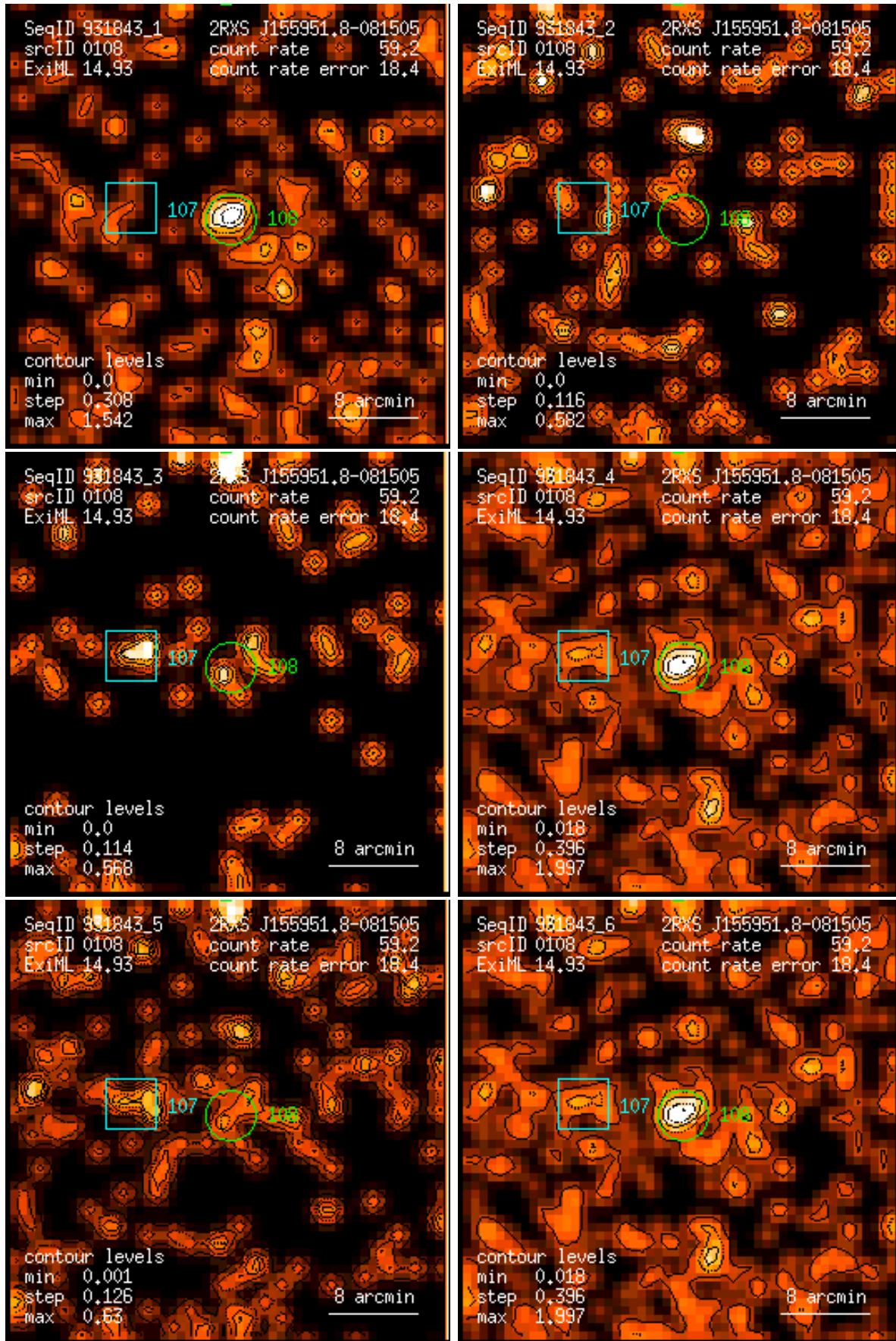
Figure 108: RASS 931843: detection 0108: band rate images, Gaussian filter: (1) PSPC channels 11 – 41, (2) 52 – 90, (3) 91 – 201, (4) 11 – 235, (5) 52 – 201, (6) 11 – 201. Broad band rates in counts/ks. Band rate contour levels in counts/ks/arcmin 2 .
