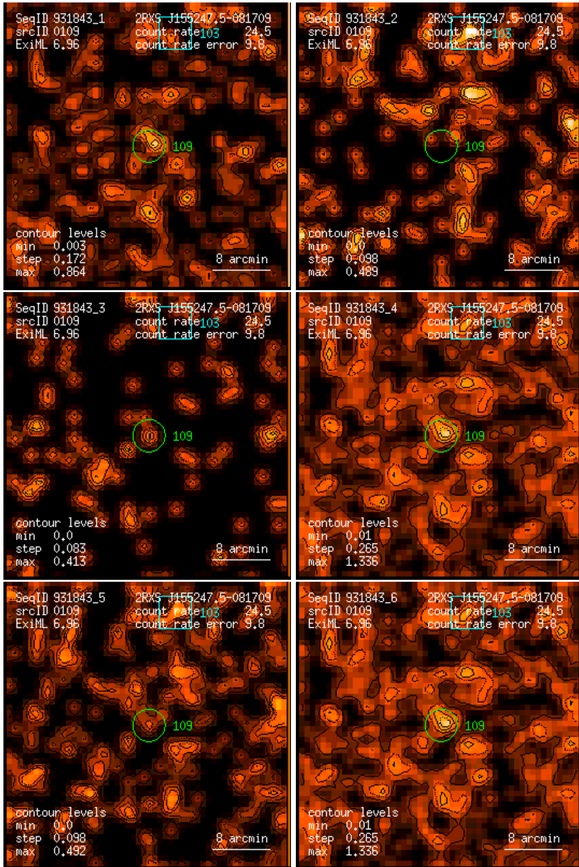
Figure 109: RASS 931843: detection 0109: band rate images, Gaussian filter: (1) PSPC channels 11 – 41, (2) 52 – 90, (3) 91 – 201, (4) 11 – 235, (5) 52 – 201, (6) 11 – 201. Broad band rates in counts/ks. Band rate contour levels in counts/ks/arcmin 2 .
