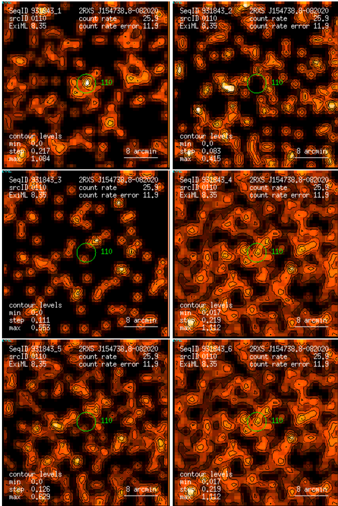
Figure 110: RASS 931843: detection 0110: band rate images, Gaussian filter: (1) PSPC channels 11 – 41, (2) 52 – 90, (3) 91 – 201, (4) 11 – 235, (5) 52 – 201, (6) 11 – 201. Broad band rates in counts/ks. Band rate contour levels in counts/ks/arcmin 2 .
