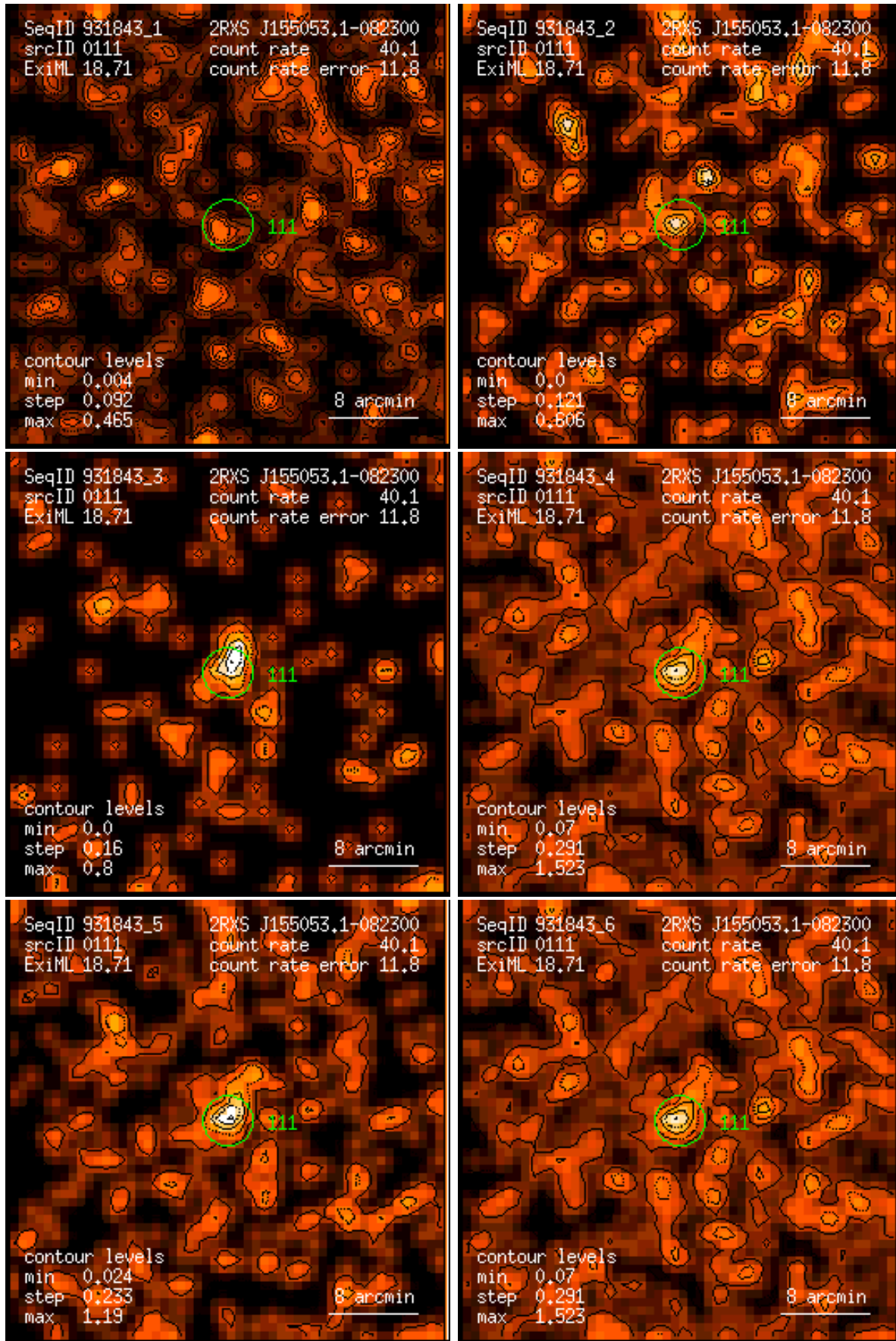
Figure 111: RASS 931843: detection 0111: band rate images, Gaussian filter: (1) PSPC channels 11 – 41, (2) 52 – 90, (3) 91 – 201, (4) 11 – 235, (5) 52 – 201, (6) 11 – 201. Broad band rates in counts/ks. Band rate contour levels in counts/ks/arcmin 2 .
