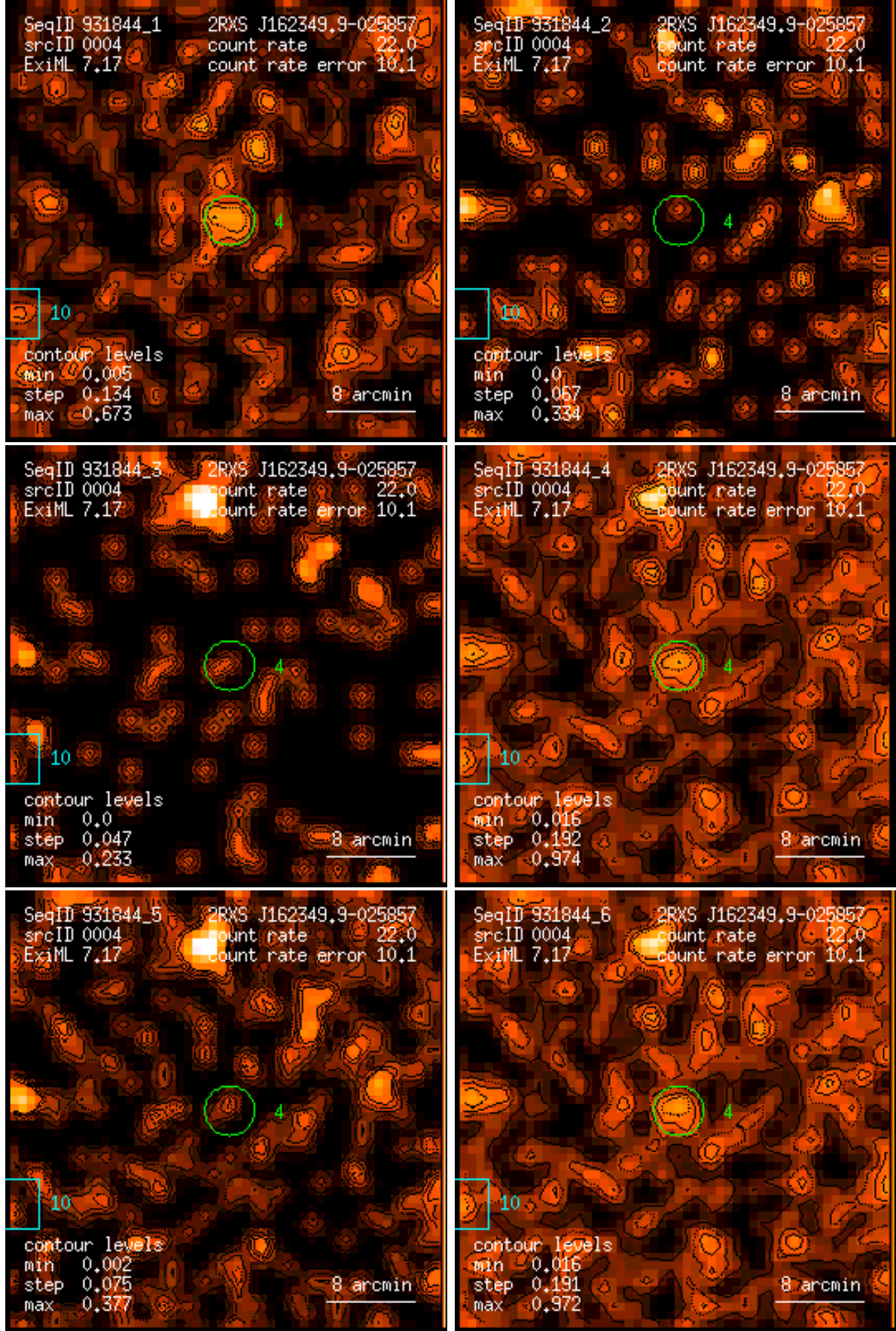
Figure 4: RASS 931844: detection 0004: band rate images, Gaussian filter: (1) PSPC channels 11 – 41, (2) 52 – 90, (3) 91 – 201, (4) 11 – 235, (5) 52 – 201, (6) 11 – 201. Broad band rates in counts/ks. Band rate contour levels in counts/ks/arcmin 2 .
