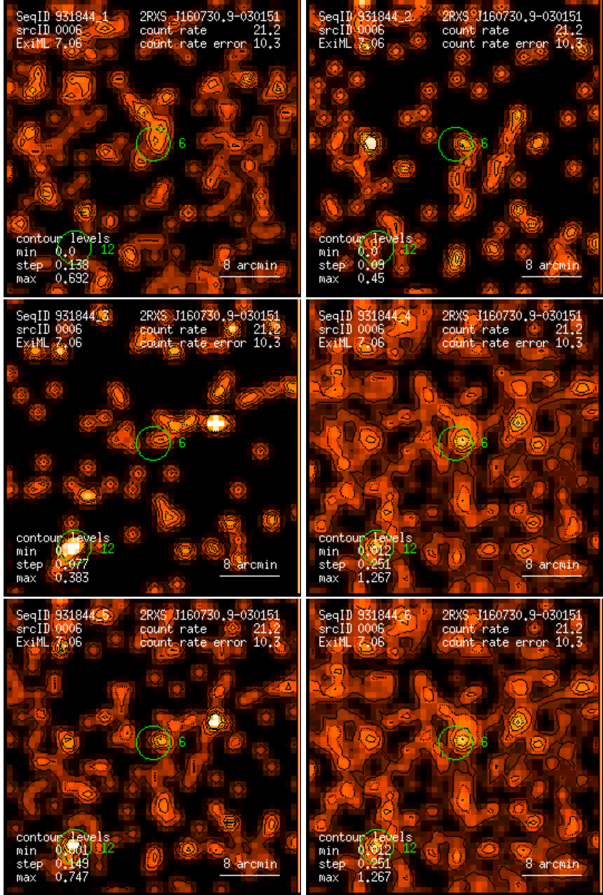
Figure 6: RASS 931844: detection 0006: band rate images, Gaussian filter: (1) PSPC channels 11 – 41, (2) 52 – 90, (3) 91 – 201, (4) 11 – 235, (5) 52 – 201, (6) 11 – 201. Broad band rates in counts/ks. Band rate contour levels in counts/ks/arcmin 2 .
