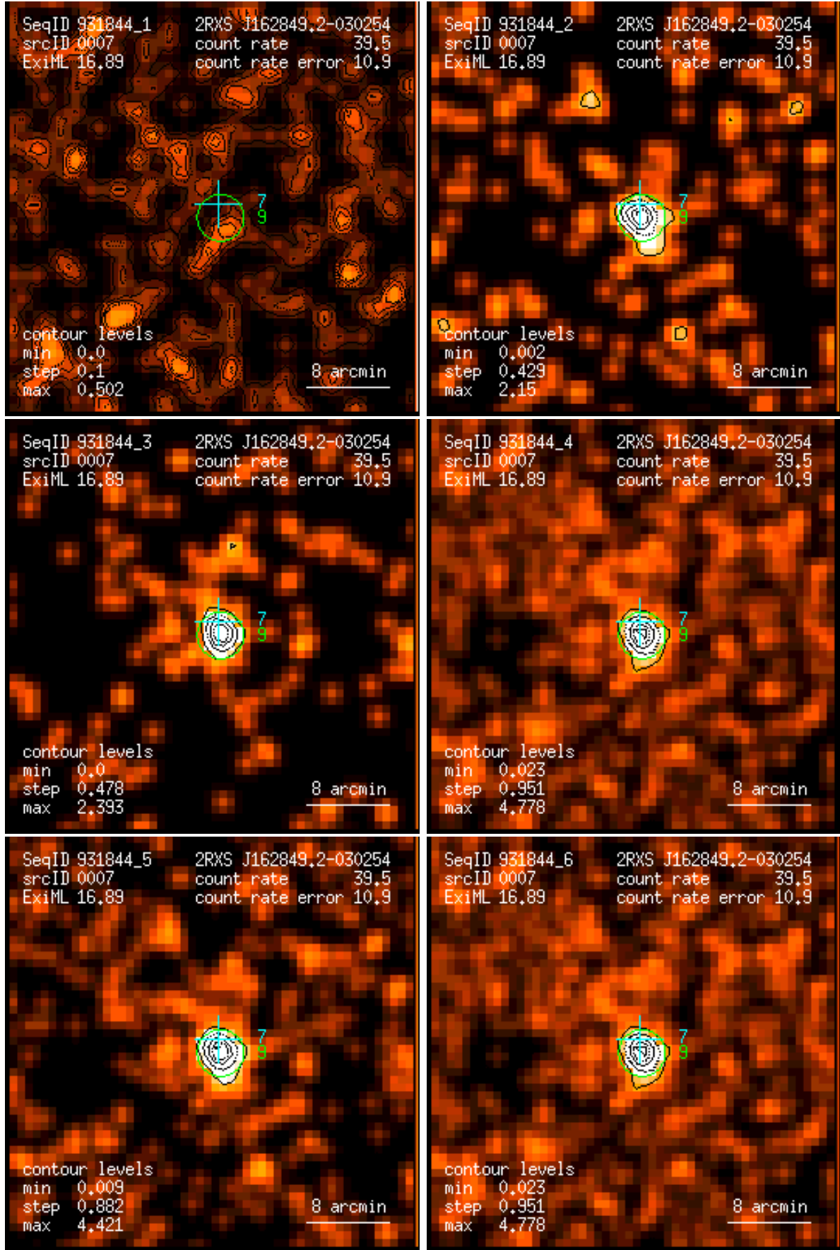
Figure 7: RASS 931844: detection 0007: band rate images, Gaussian filter: (1) PSPC channels 11 – 41, (2) 52 – 90, (3) 91 – 201, (4) 11 – 235, (5) 52 – 201, (6) 11 – 201. Broad band rates in counts/ks. Band rate contour levels in counts/ks/arcmin 2 .
