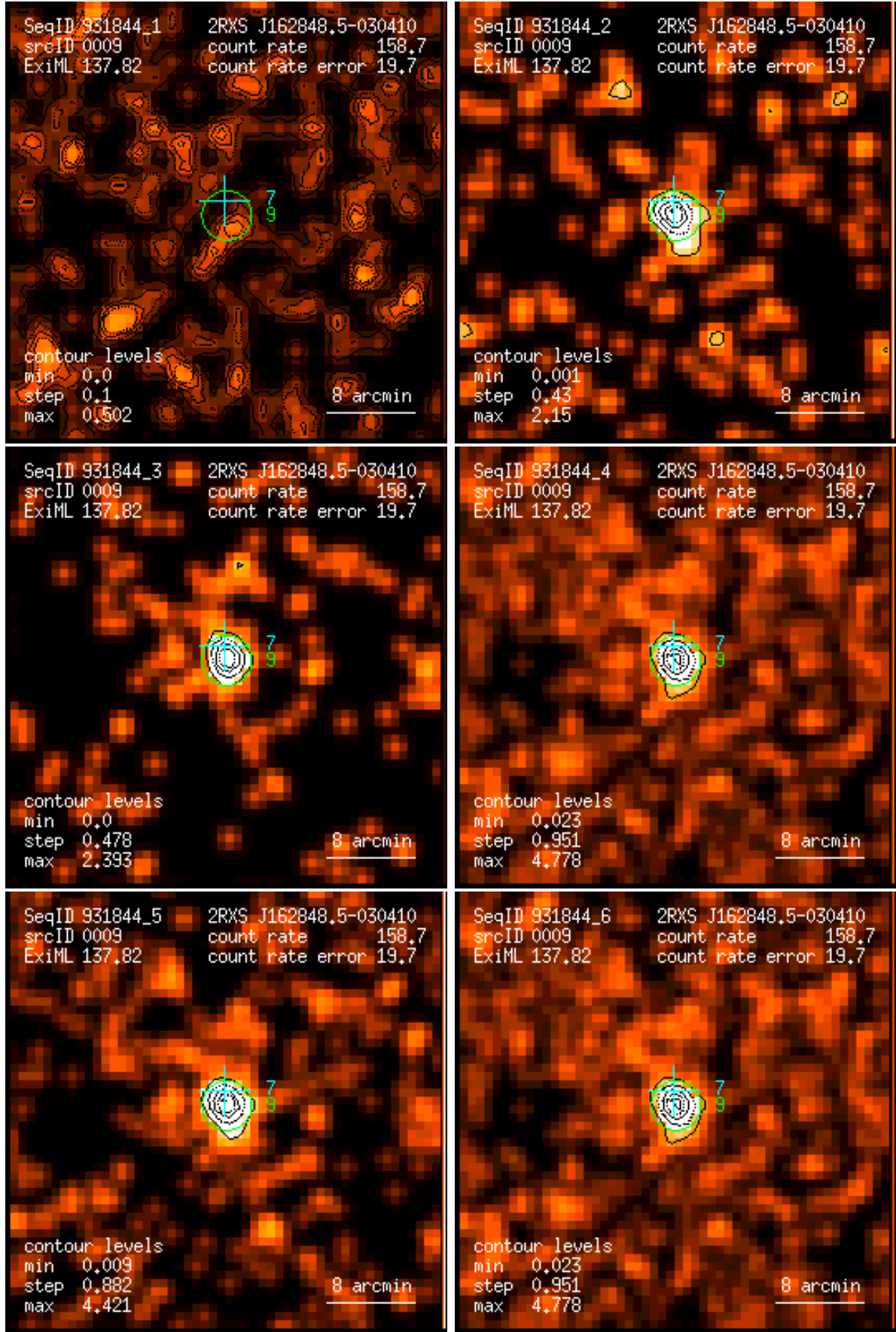
Figure 9: RASS 931844: detection 0009: band rate images, Gaussian filter: (1) PSPC channels 11 – 41, (2) 52 – 90, (3) 91 – 201, (4) 11 – 235, (5) 52 – 201, (6) 11 – 201. Broad band rates in counts/ks. Band rate contour levels in counts/ks/arcmin 2 .
