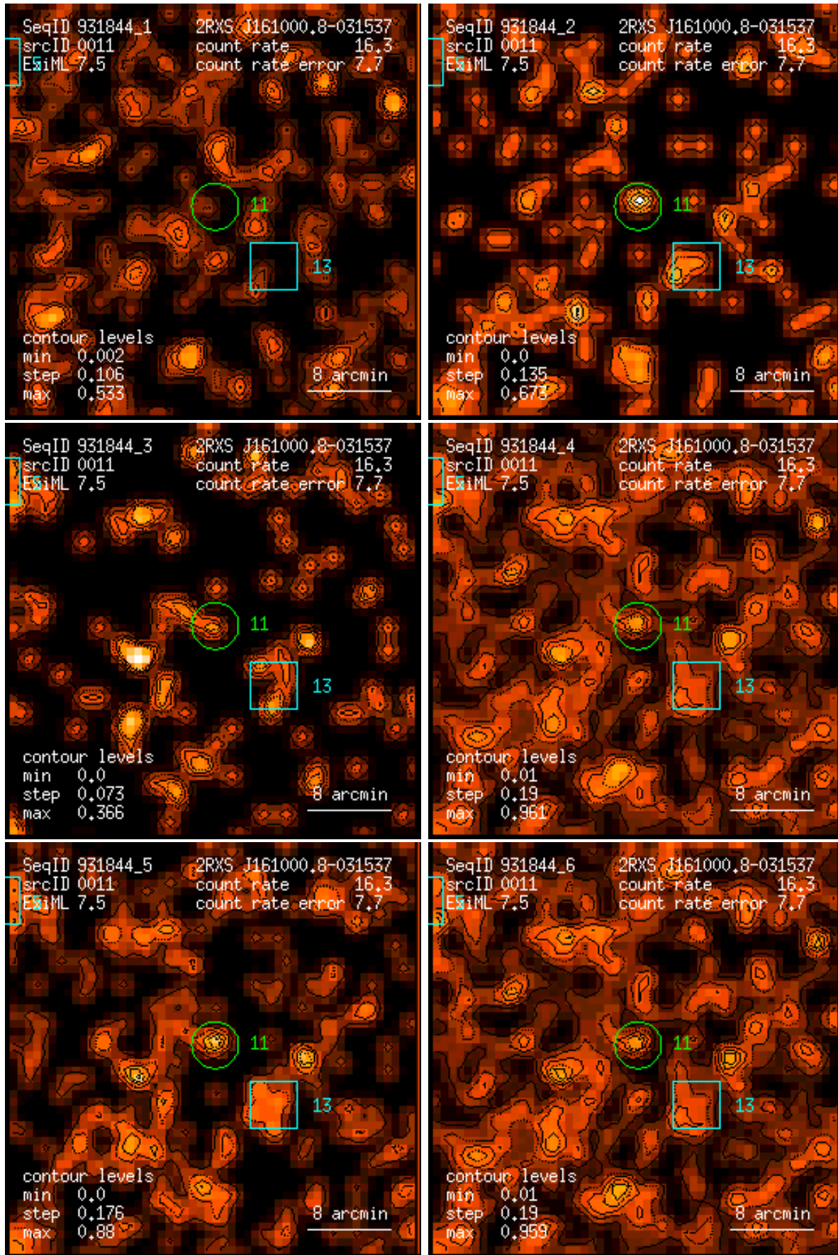
Figure 11: RASS 931844: detection 0011: band rate images, Gaussian filter: (1) PSPC channels 11 – 41, (2) 52 – 90, (3) 91 – 201, (4) 11 – 235, (5) 52 – 201, (6) 11 – 201. Broad band rates in counts/ks. Band rate contour levels in counts/ks/arcmin 2 .
