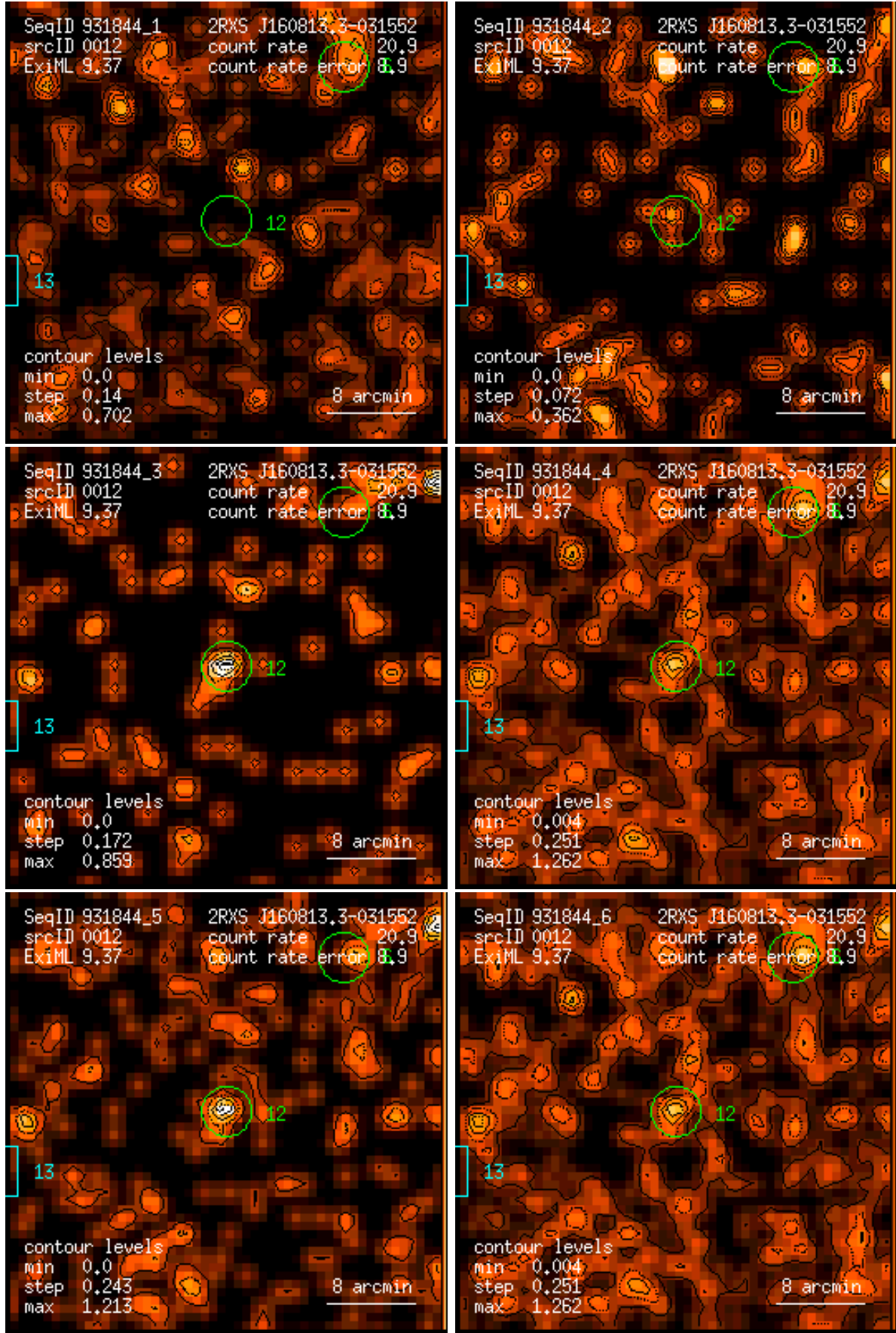
Figure 12: RASS 931844: detection 0012: band rate images, Gaussian filter: (1) PSPC channels 11 – 41, (2) 52 – 90, (3) 91 – 201, (4) 11 – 235, (5) 52 – 201, (6) 11 – 201. Broad band rates in counts/ks. Band rate contour levels in counts/ks/arcmin 2 .
