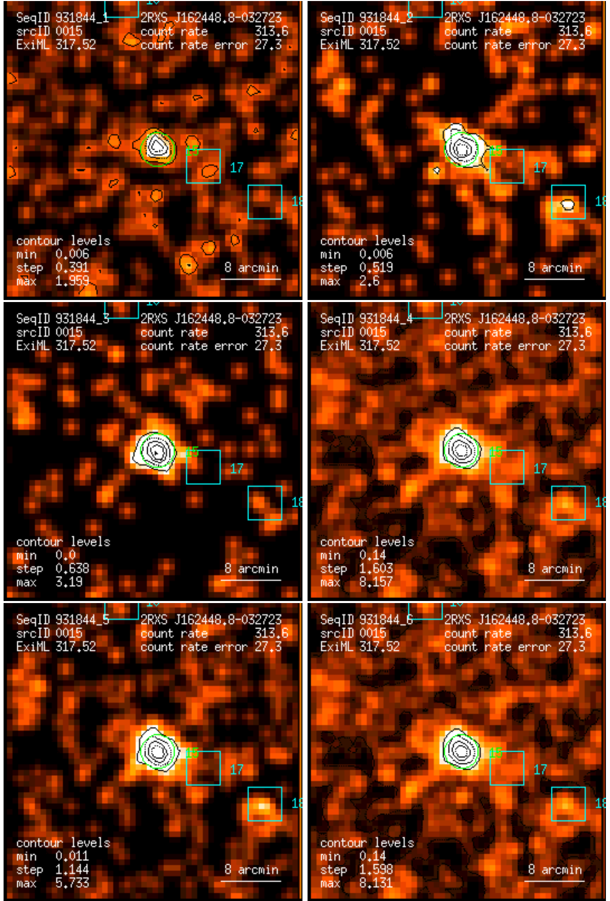
Figure 15: RASS 931844: detection 0015: band rate images, Gaussian filter: (1) PSPC channels 11 – 41, (2) 52 – 90, (3) 91 – 201, (4) 11 – 235, (5) 52 – 201, (6) 11 – 201. Broad band rates in counts/ks. Band rate contour levels in counts/ks/arcmin 2 .
