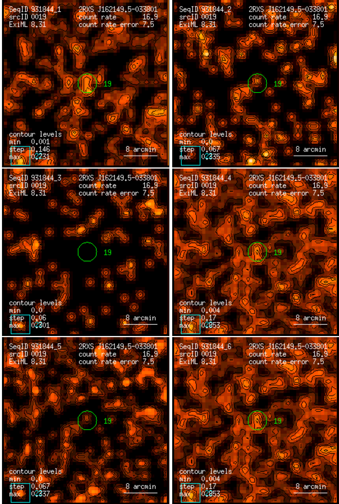
Figure 19: RASS 931844: detection 0019: band rate images, Gaussian filter: (1) PSPC channels 11 – 41, (2) 52 – 90, (3) 91 – 201, (4) 11 – 235, (5) 52 – 201, (6) 11 – 201. Broad band rates in counts/ks. Band rate contour levels in counts/ks/arcmin 2 .
