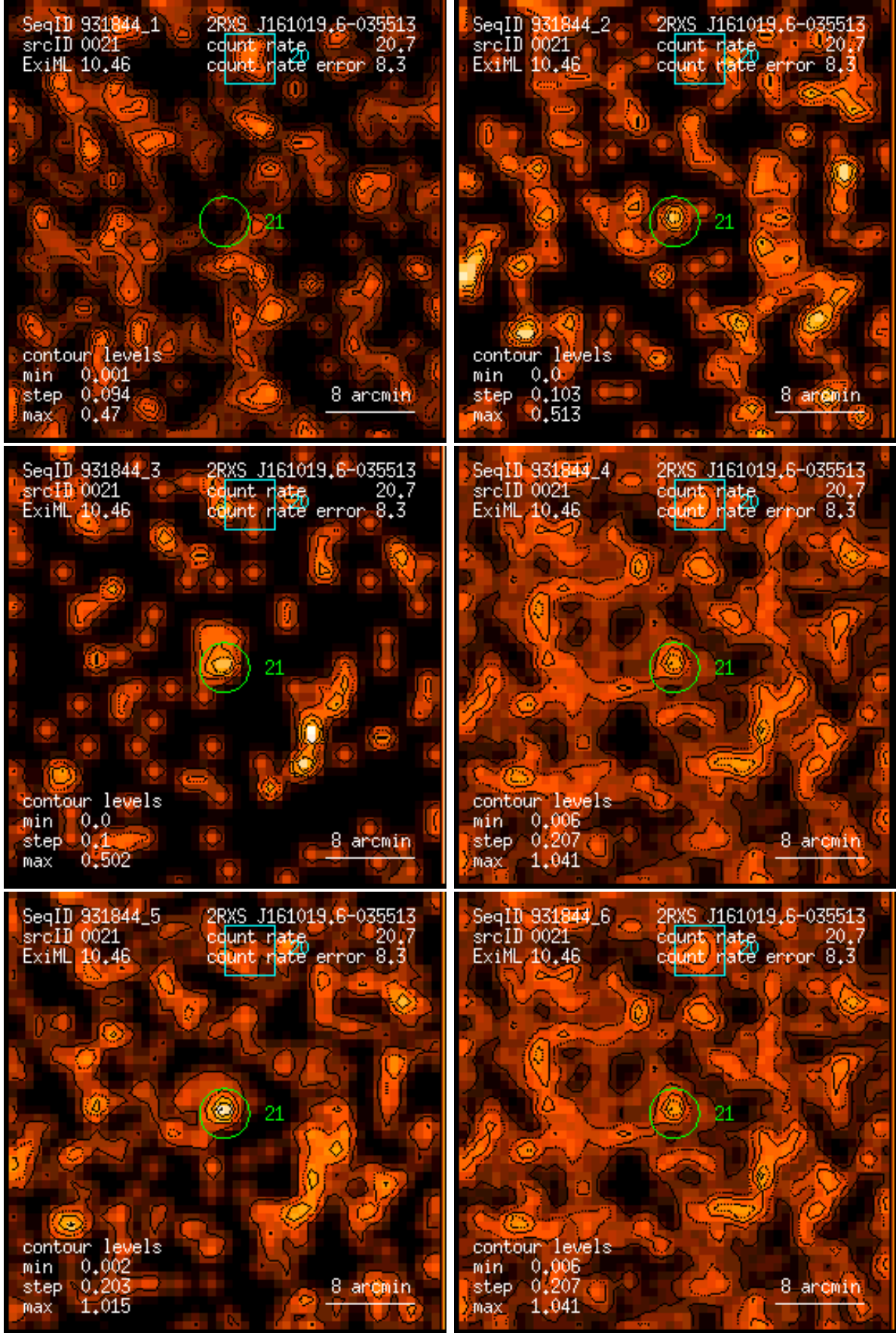
Figure 21: RASS 931844: detection 0021: band rate images, Gaussian filter: (1) PSPC channels 11 – 41, (2) 52 – 90, (3) 91 – 201, (4) 11 – 235, (5) 52 – 201, (6) 11 – 201. Broad band rates in counts/ks. Band rate contour levels in counts/ks/arcmin 2 .
