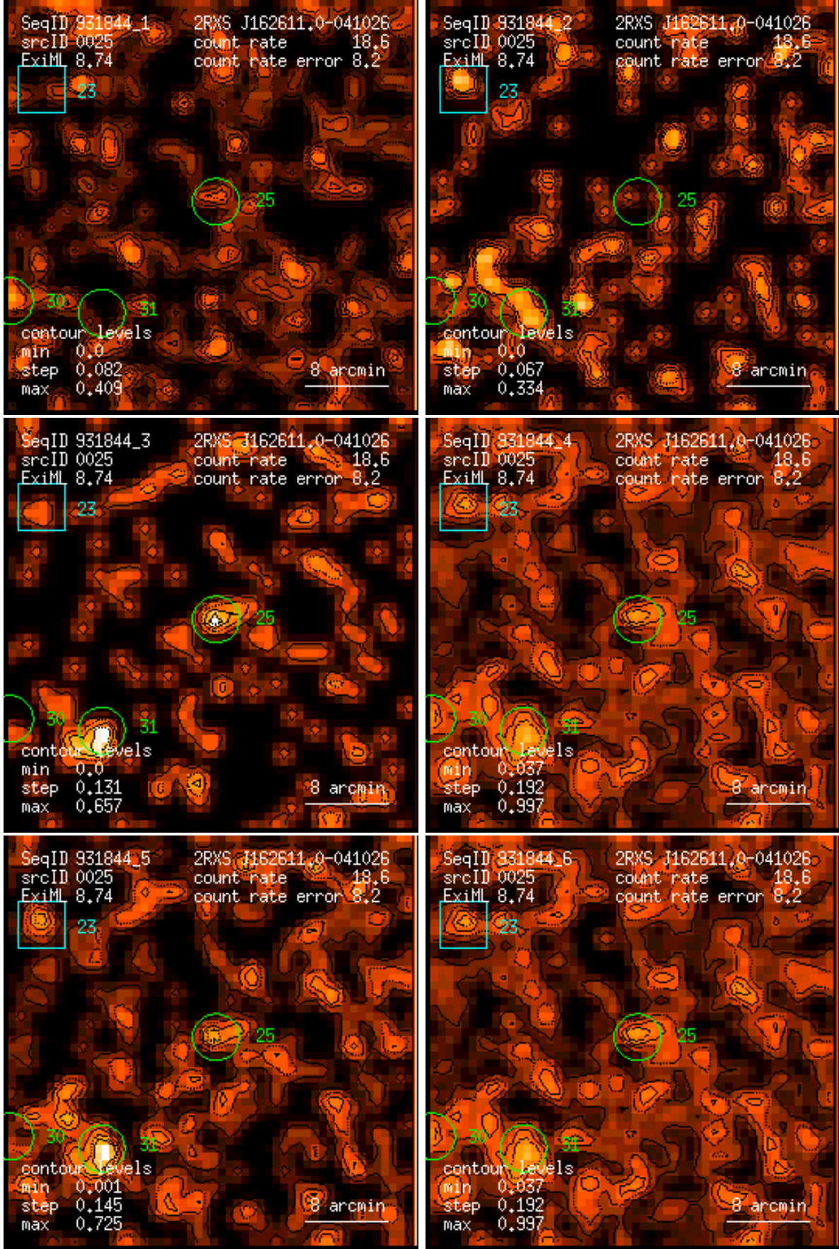
Figure 25: RASS 931844: detection 0025: band rate images, Gaussian filter: (1) PSPC channels 11 – 41, (2) 52 – 90, (3) 91 – 201, (4) 11 – 235, (5) 52 – 201, (6) 11 – 201. Broad band rates in counts/ks. Band rate contour levels in counts/ks/arcmin 2 .
