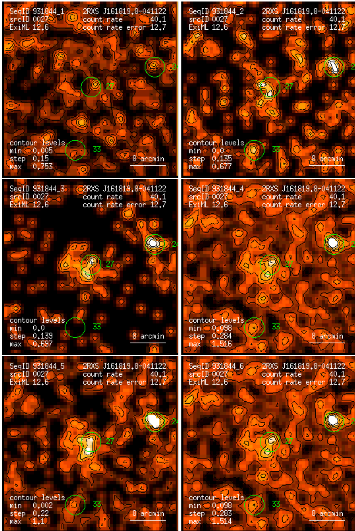
Figure 27: RASS 931844: detection 0027: band rate images, Gaussian filter: (1) PSPC channels 11 – 41, (2) 52 – 90, (3) 91 – 201, (4) 11 – 235, (5) 52 – 201, (6) 11 – 201. Broad band rates in counts/ks. Band rate contour levels in counts/ks/arcmin 2 .
