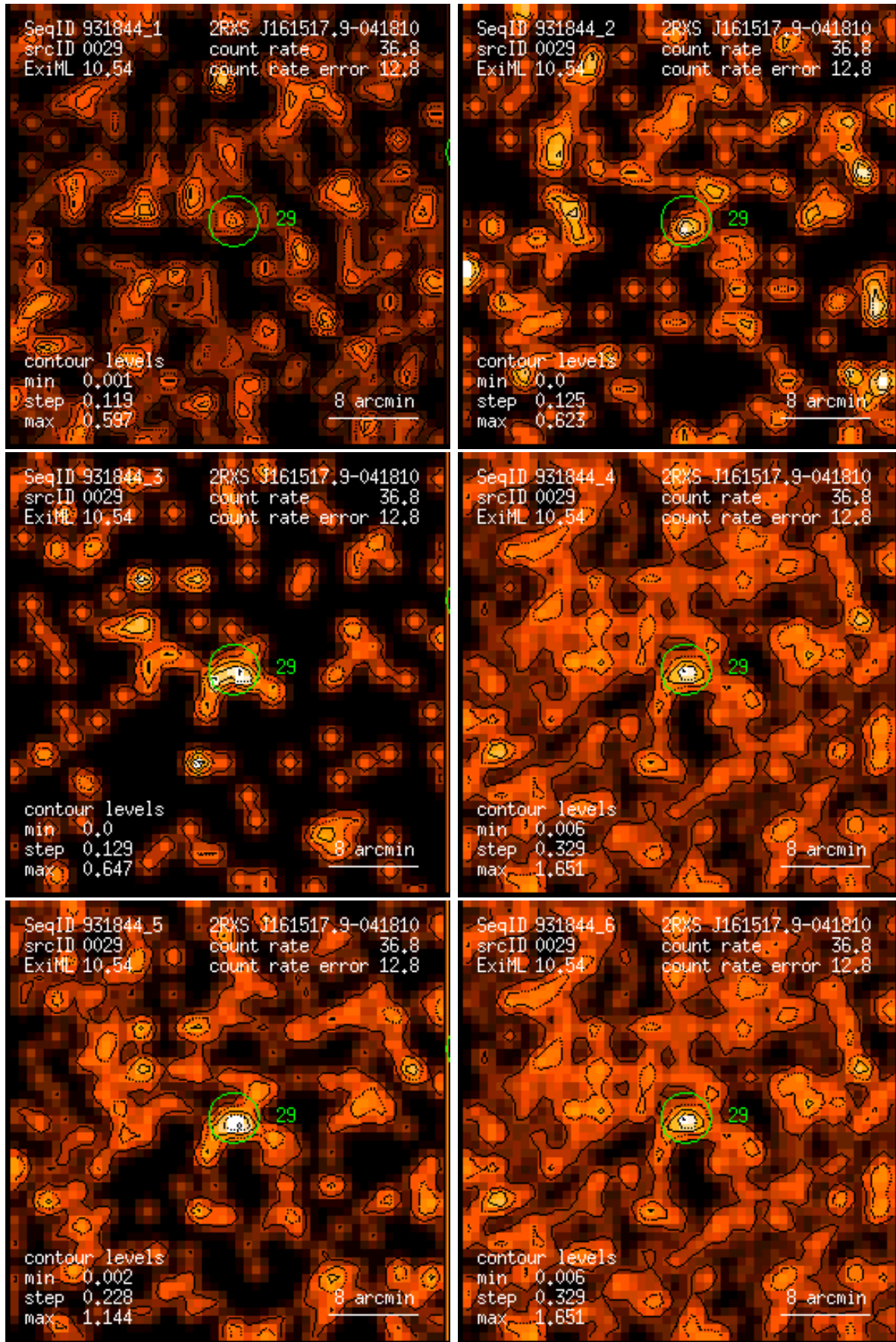
Figure 29: RASS 931844: detection 0029: band rate images, Gaussian filter: (1) PSPC channels 11 – 41, (2) 52 – 90, (3) 91 – 201, (4) 11 – 235, (5) 52 – 201, (6) 11 – 201. Broad band rates in counts/ks. Band rate contour levels in counts/ks/arcmin 2 .
