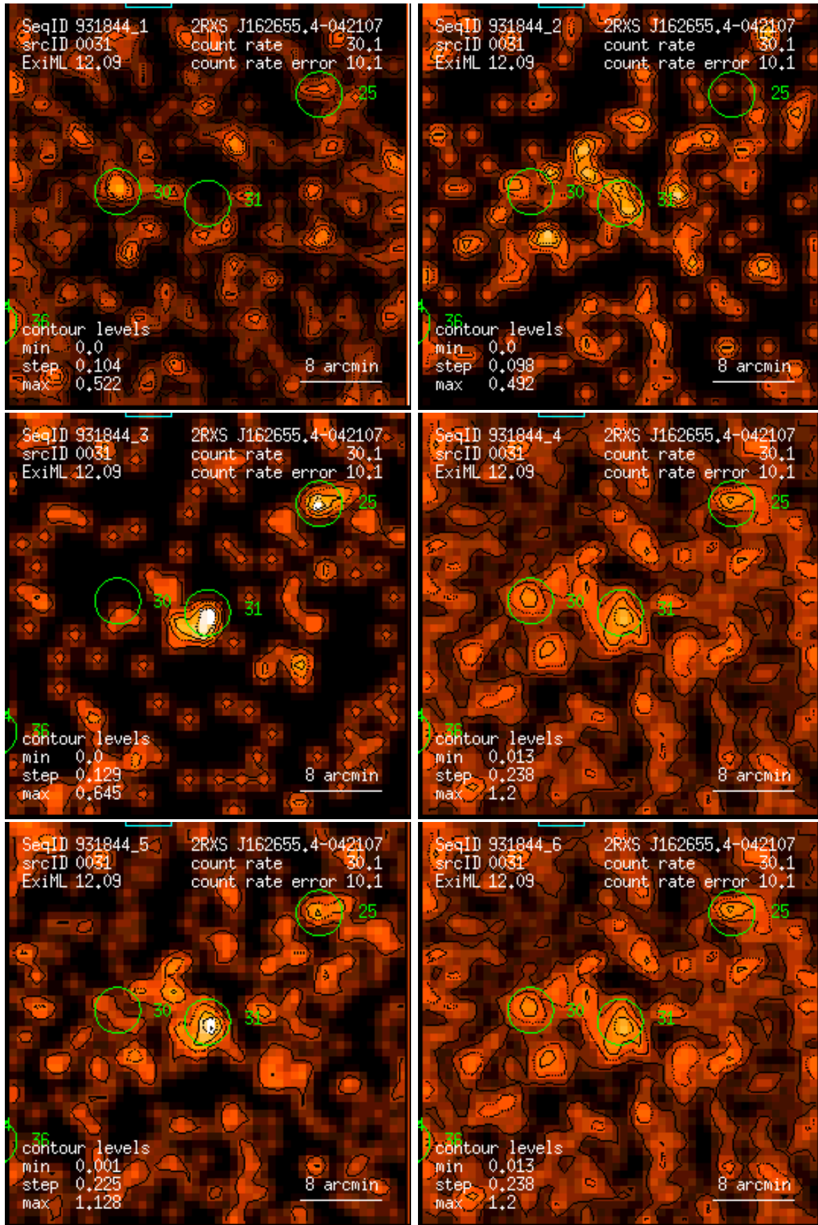
Figure 31: RASS 931844: detection 0031: band rate images, Gaussian filter: (1) PSPC channels 11 – 41, (2) 52 – 90, (3) 91 – 201, (4) 11 – 235, (5) 52 – 201, (6) 11 – 201. Broad band rates in counts/ks. Band rate contour levels in counts/ks/arcmin 2 .
