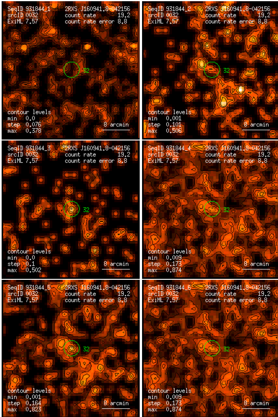
Figure 32: RASS 931844: detection 0032: band rate images, Gaussian filter: (1) PSPC channels 11 – 41, (2) 52 – 90, (3) 91 – 201, (4) 11 – 235, (5) 52 – 201, (6) 11 – 201. Broad band rates in counts/ks. Band rate contour levels in counts/ks/arcmin 2 .
