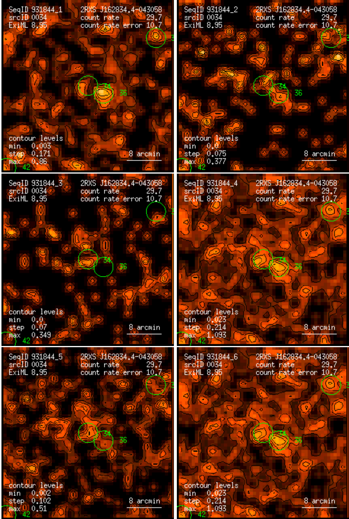
Figure 34: RASS 931844: detection 0034: band rate images, Gaussian filter: (1) PSPC channels 11 – 41, (2) 52 – 90, (3) 91 – 201, (4) 11 – 235, (5) 52 – 201, (6) 11 – 201. Broad band rates in counts/ks. Band rate contour levels in counts/ks/arcmin 2 .
