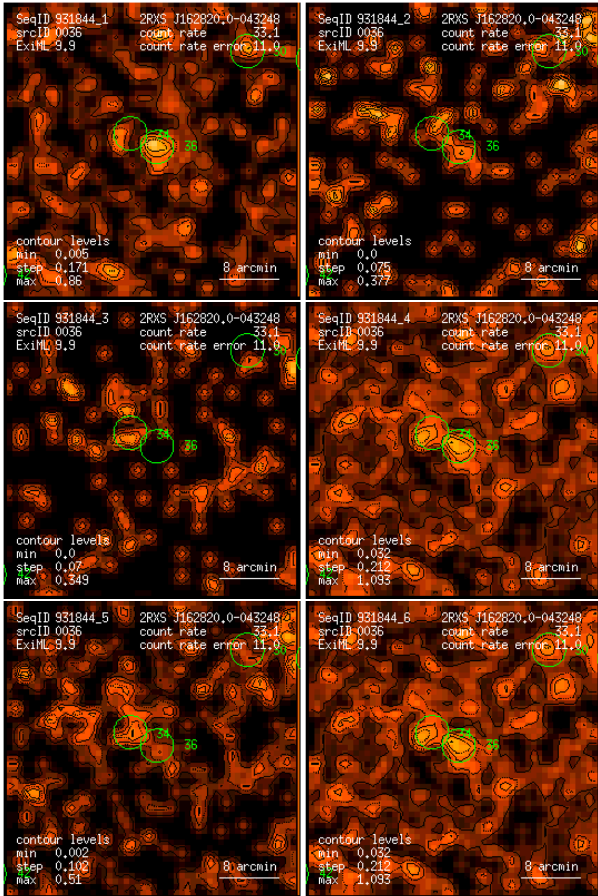
Figure 36: RASS 931844: detection 0036: band rate images, Gaussian filter: (1) PSPC channels 11 – 41, (2) 52 – 90, (3) 91 – 201, (4) 11 – 235, (5) 52 – 201, (6) 11 – 201. Broad band rates in counts/ks. Band rate contour levels in counts/ks/arcmin 2 .
