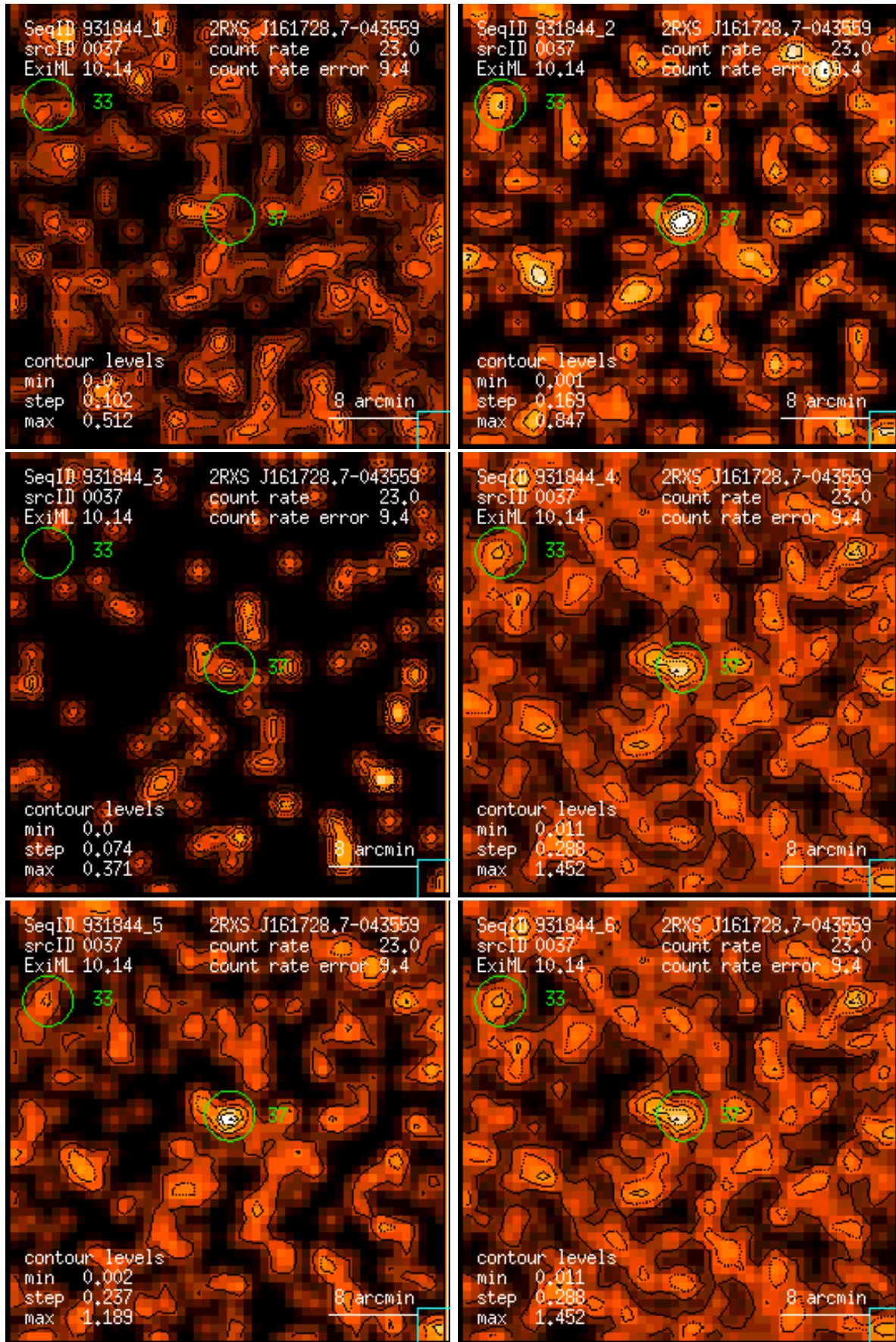
Figure 37: RASS 931844: detection 0037: band rate images, Gaussian filter: (1) PSPC channels 11 – 41, (2) 52 – 90, (3) 91 – 201, (4) 11 – 235, (5) 52 – 201, (6) 11 – 201. Broad band rates in counts/ks. Band rate contour levels in counts/ks/arcmin 2 .
