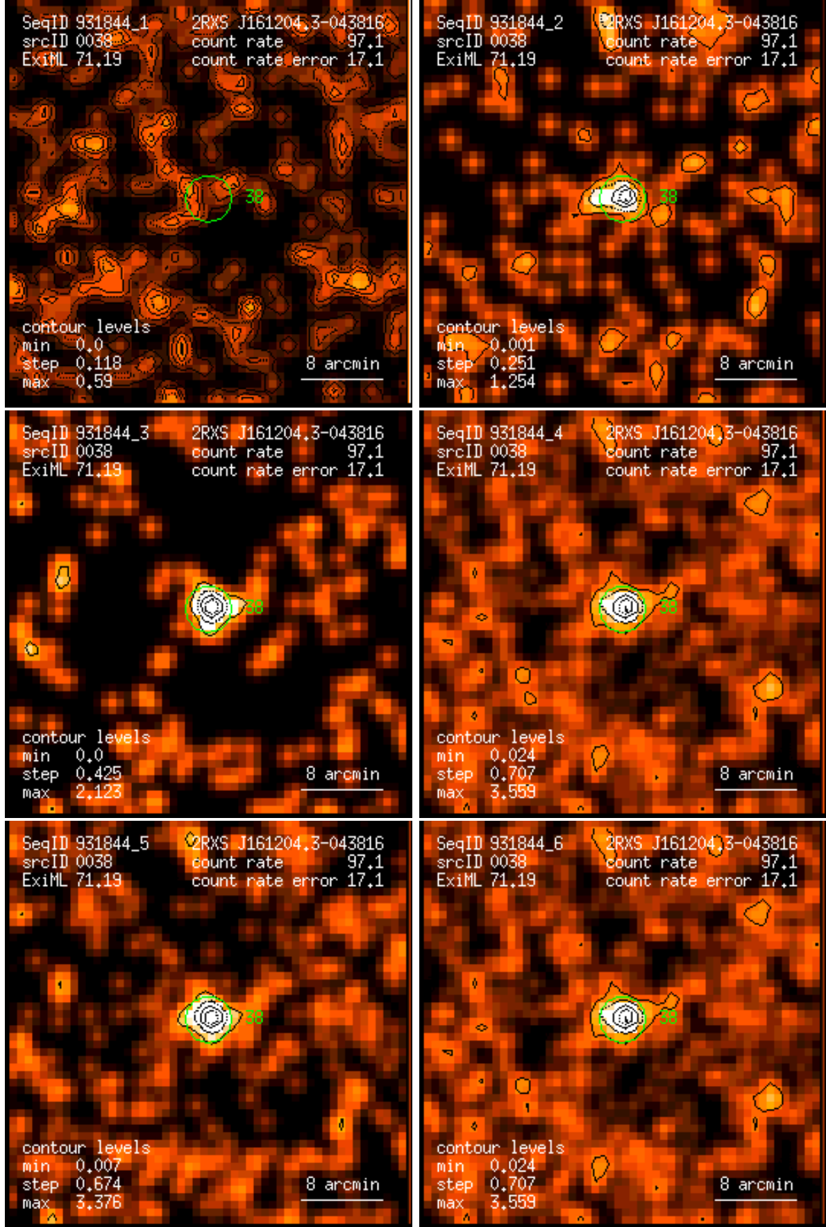
Figure 38: RASS 931844: detection 0038: band rate images, Gaussian filter: (1) PSPC channels 11 – 41, (2) 52 – 90, (3) 91 – 201, (4) 11 – 235, (5) 52 – 201, (6) 11 – 201. Broad band rates in counts/ks. Band rate contour levels in counts/ks/arcmin 2 .
