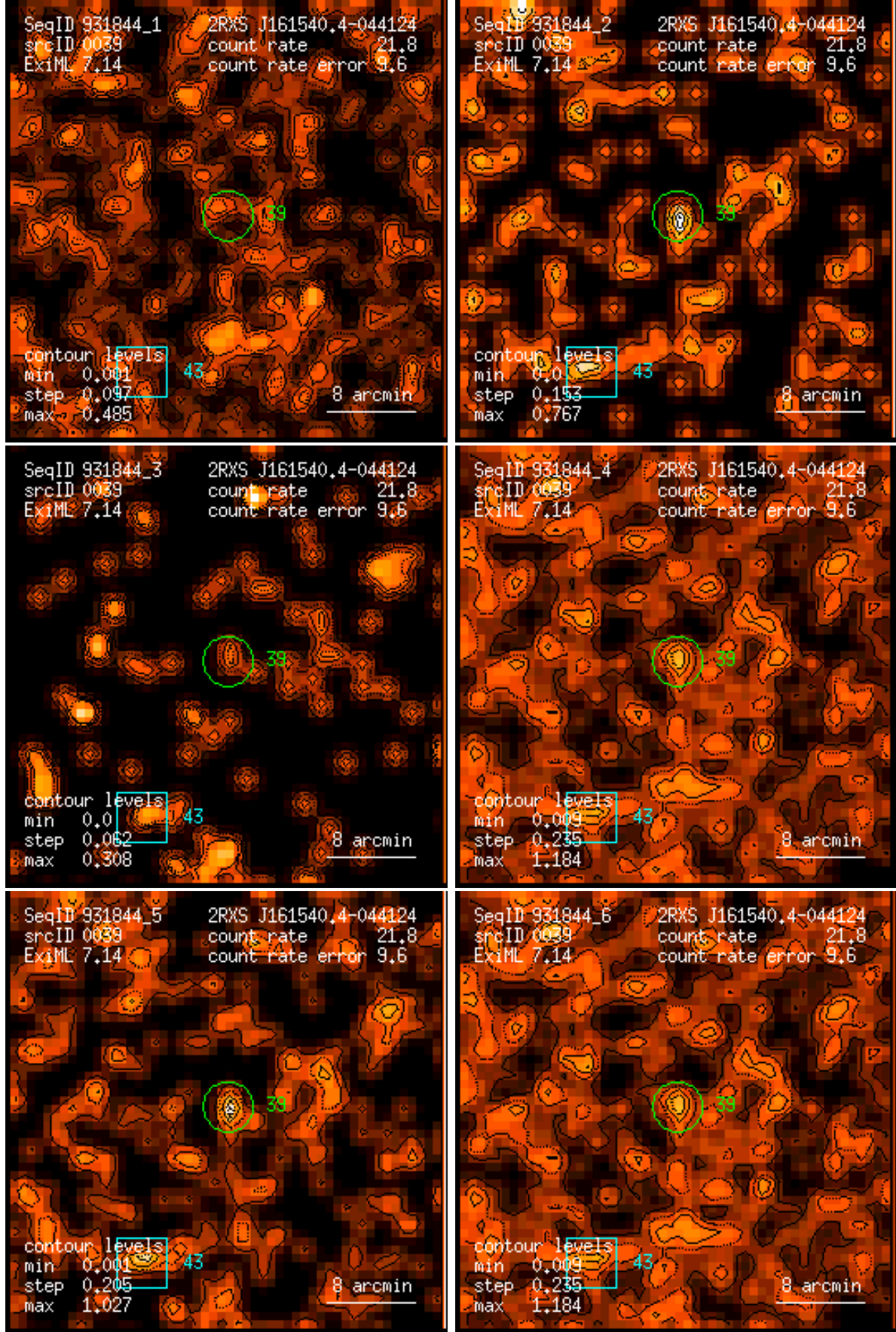
Figure 39: RASS 931844: detection 0039: band rate images, Gaussian filter: (1) PSPC channels 11 – 41, (2) 52 – 90, (3) 91 – 201, (4) 11 – 235, (5) 52 – 201, (6) 11 – 201. Broad band rates in counts/ks. Band rate contour levels in counts/ks/arcmin 2 .
