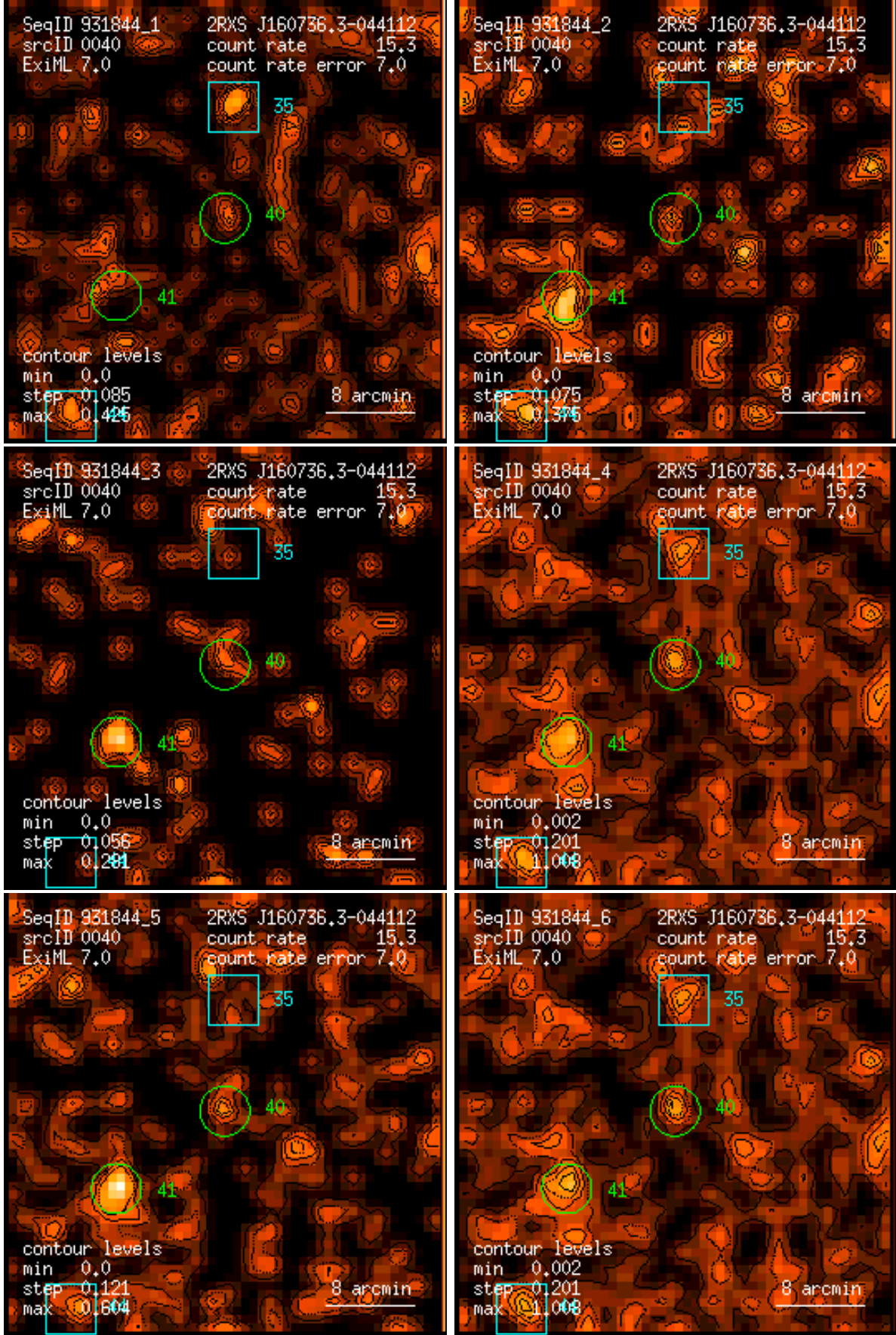
Figure 40: RASS 931844: detection 0040: band rate images, Gaussian filter: (1) PSPC channels 11 – 41, (2) 52 – 90, (3) 91 – 201, (4) 11 – 235, (5) 52 – 201, (6) 11 – 201. Broad band rates in counts/ks. Band rate contour levels in counts/ks/arcmin 2 .
