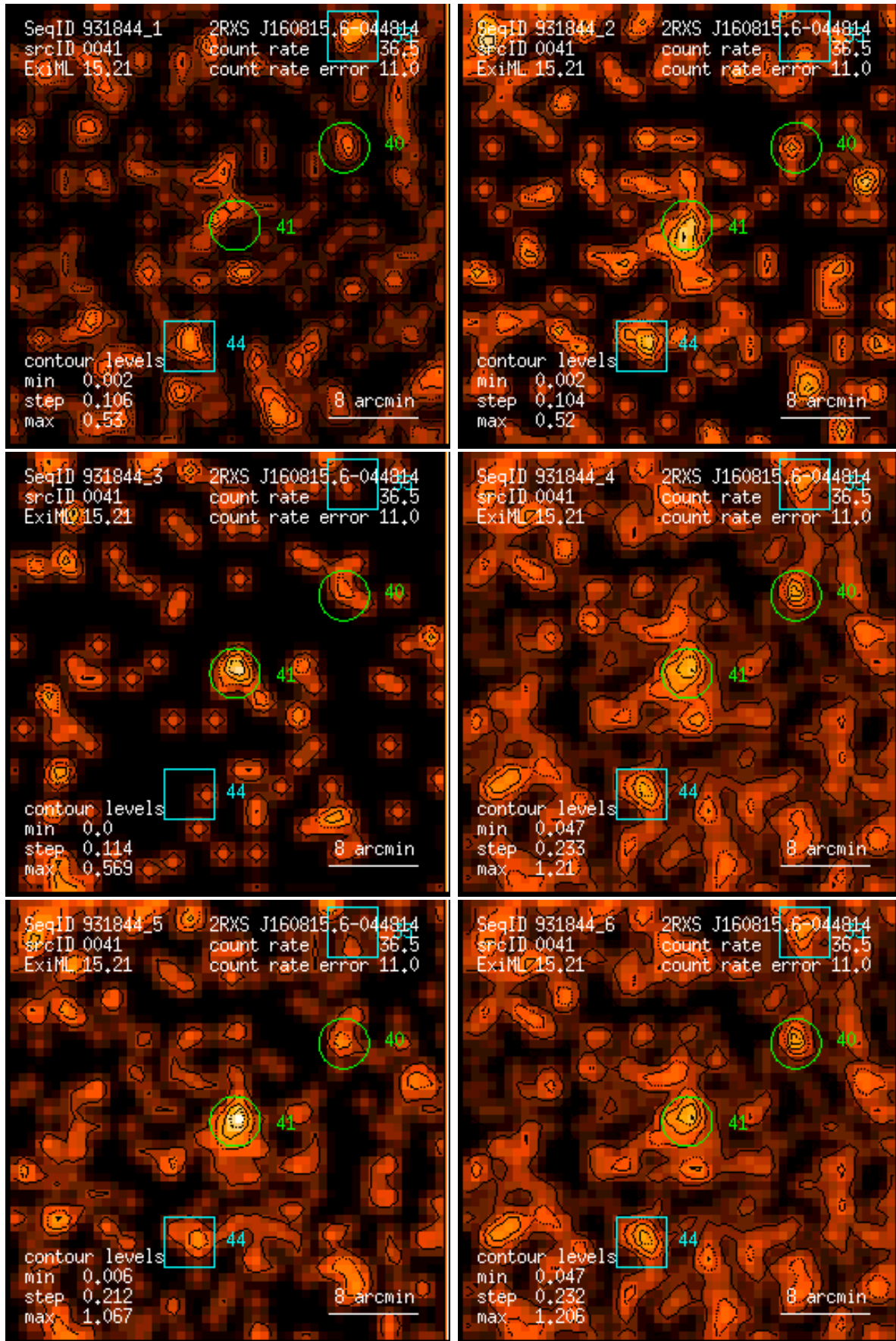
Figure 41: RASS 931844: detection 0041: band rate images, Gaussian filter: (1) PSPC channels 11 – 41, (2) 52 – 90, (3) 91 – 201, (4) 11 – 235, (5) 52 – 201, (6) 11 – 201. Broad band rates in counts/ks. Band rate contour levels in counts/ks/arcmin 2 .
