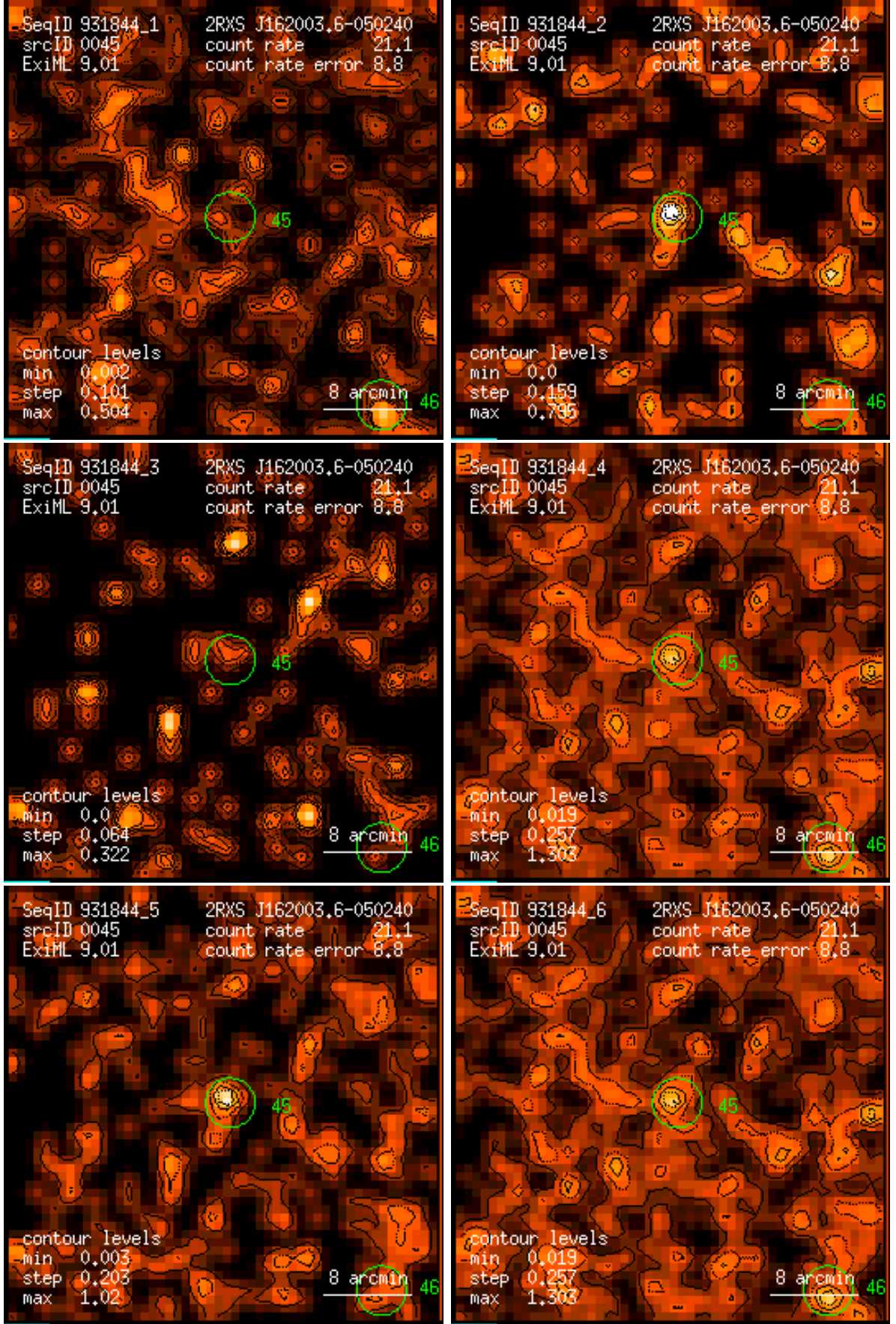
Figure 45: RASS 931844: detection 0045: band rate images, Gaussian filter: (1) PSPC channels 11 – 41, (2) 52 – 90, (3) 91 – 201, (4) 11 – 235, (5) 52 – 201, (6) 11 – 201. Broad band rates in counts/ks. Band rate contour levels in counts/ks/arcmin 2 .
