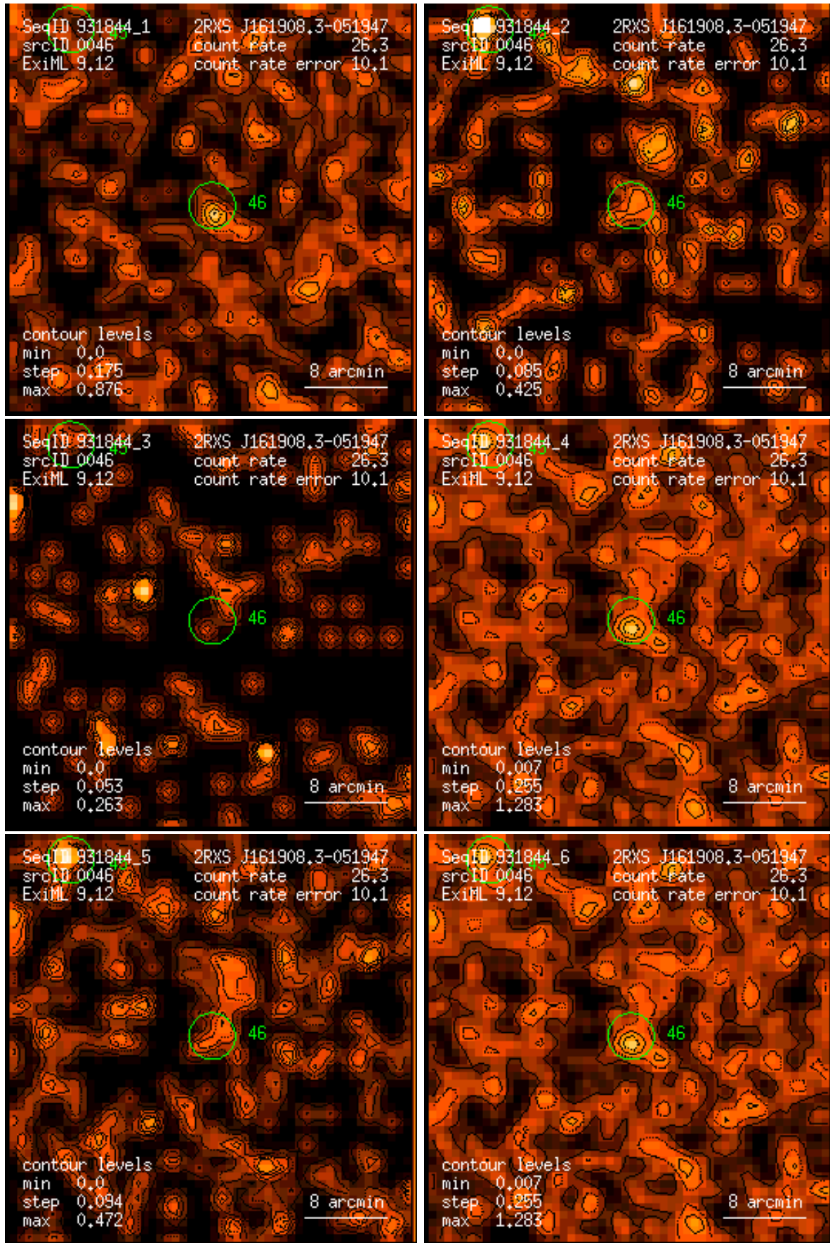
Figure 46: RASS 931844: detection 0046: band rate images, Gaussian filter: (1) PSPC channels 11 – 41, (2) 52 – 90, (3) 91 – 201, (4) 11 – 235, (5) 52 – 201, (6) 11 – 201. Broad band rates in counts/ks. Band rate contour levels in counts/ks/arcmin 2 .
