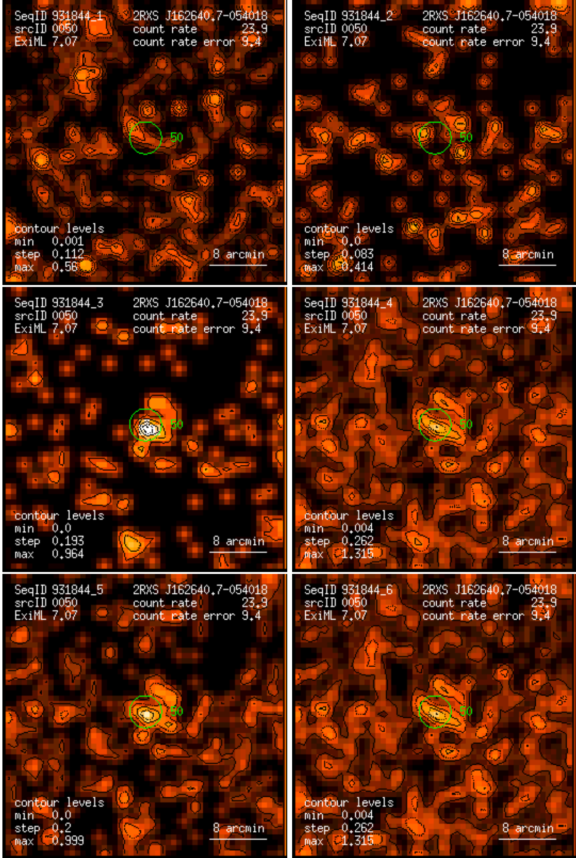
Figure 50: RASS 931844: detection 0050: band rate images, Gaussian filter: (1) PSPC channels 11 – 41, (2) 52 – 90, (3) 91 – 201, (4) 11 – 235, (5) 52 – 201, (6) 11 – 201. Broad band rates in counts/ks. Band rate contour levels in counts/ks/arcmin 2 .
