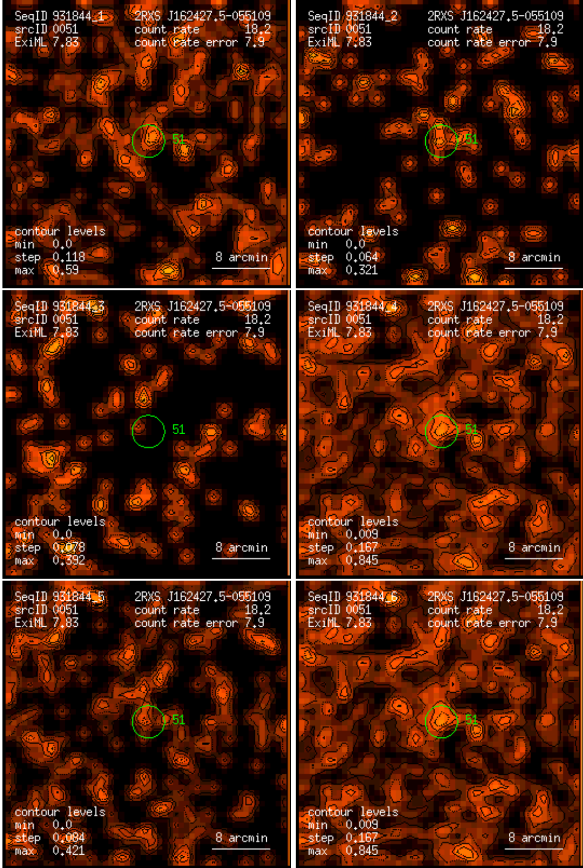
Figure 51: RASS 931844: detection 0051: band rate images, Gaussian filter: (1) PSPC channels 11 – 41, (2) 52 – 90, (3) 91 – 201, (4) 11 – 235, (5) 52 – 201, (6) 11 – 201. Broad band rates in counts/ks. Band rate contour levels in counts/ks/arcmin 2 .
