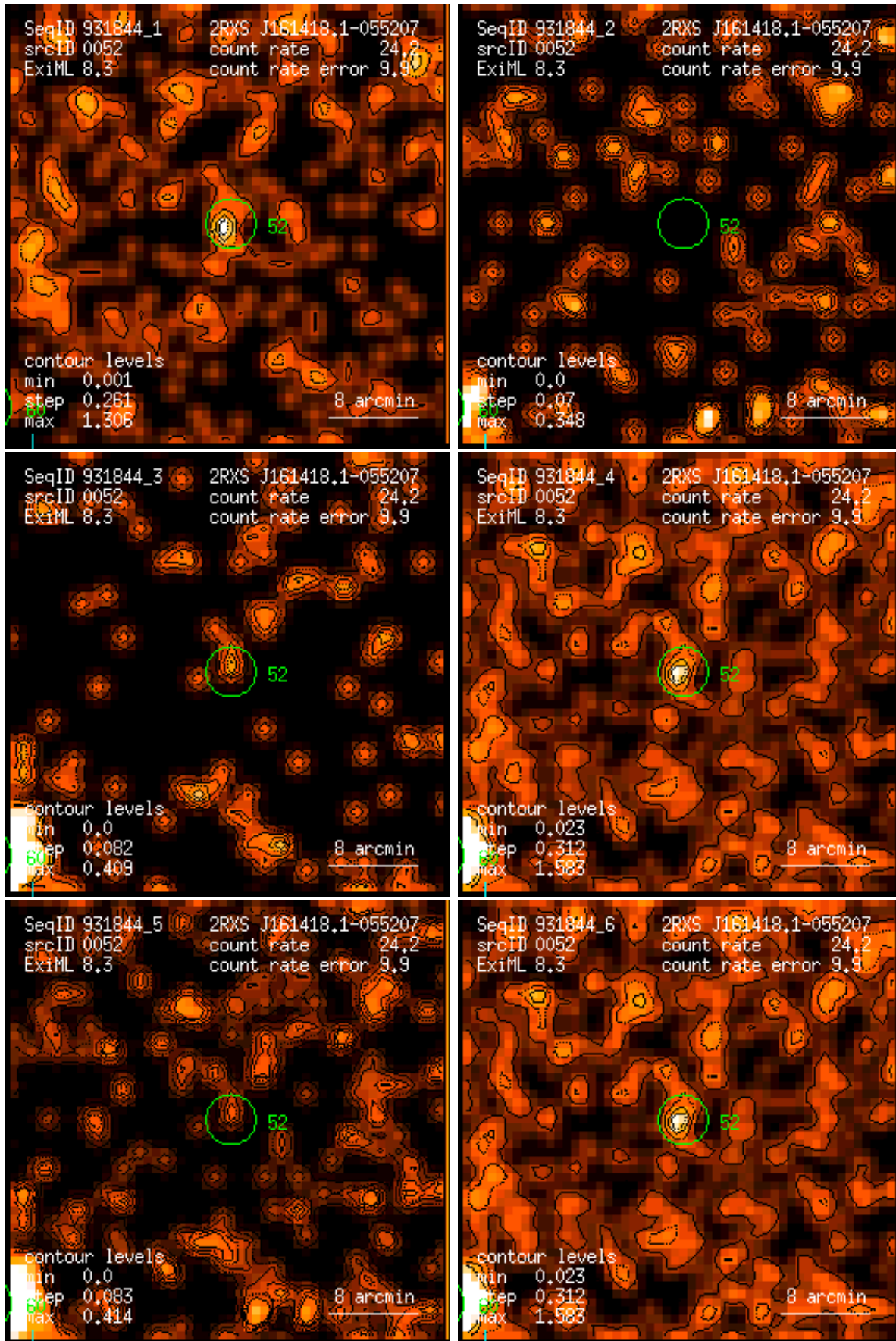
Figure 52: RASS 931844: detection 0052: band rate images, Gaussian filter: (1) PSPC channels 11 – 41, (2) 52 – 90, (3) 91 – 201, (4) 11 – 235, (5) 52 – 201, (6) 11 – 201. Broad band rates in counts/ks. Band rate contour levels in counts/ks/arcmin 2 .
