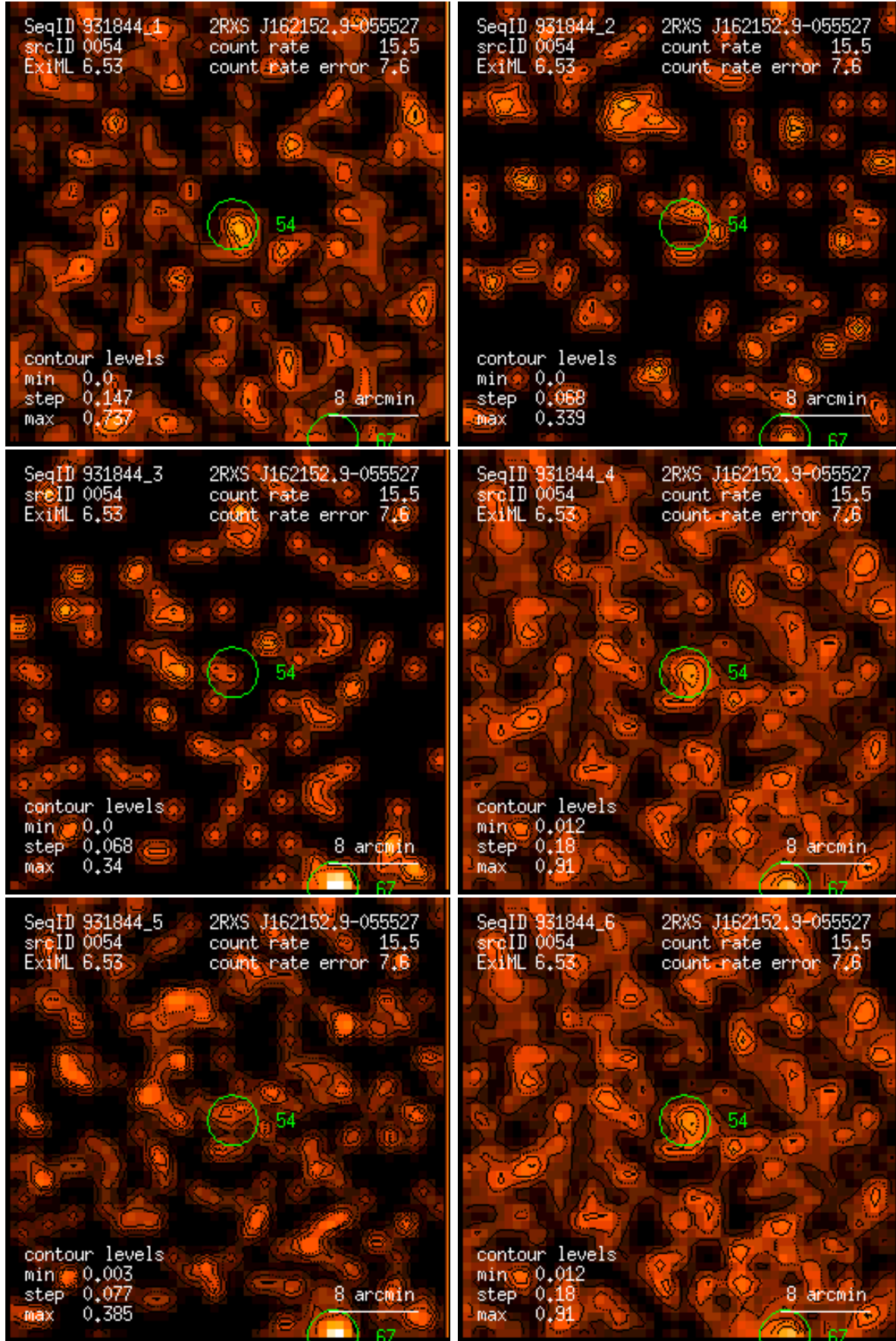
Figure 54: RASS 931844: detection 0054: band rate images, Gaussian filter: (1) PSPC channels 11 – 41, (2) 52 – 90, (3) 91 – 201, (4) 11 – 235, (5) 52 – 201, (6) 11 – 201. Broad band rates in counts/ks. Band rate contour levels in counts/ks/arcmin 2 .
