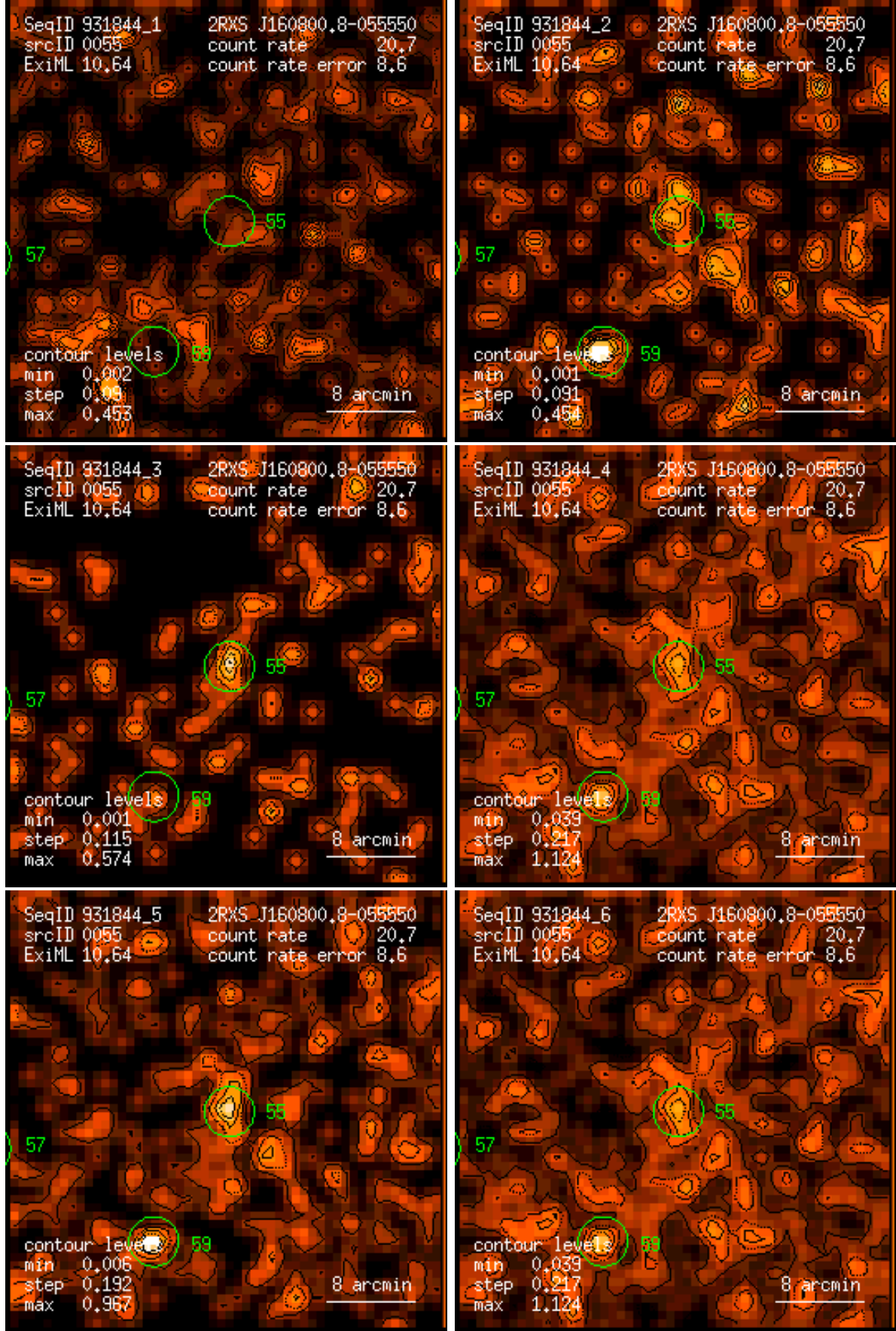
Figure 55: RASS 931844: detection 0055: band rate images, Gaussian filter: (1) PSPC channels 11 – 41, (2) 52 – 90, (3) 91 – 201, (4) 11 – 235, (5) 52 – 201, (6) 11 – 201. Broad band rates in counts/ks. Band rate contour levels in counts/ks/arcmin 2 .
