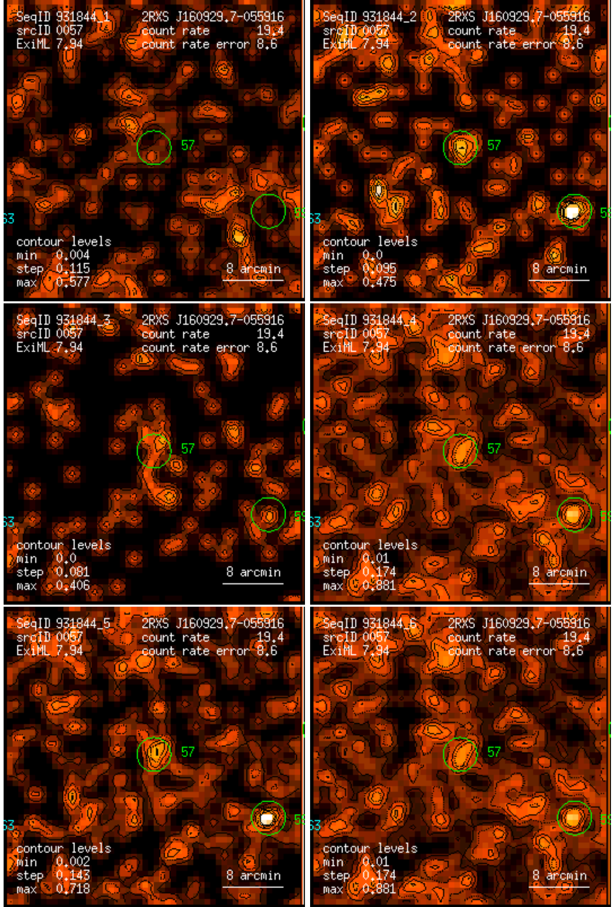
Figure 57: RASS 931844: detection 0057: band rate images, Gaussian filter: (1) PSPC channels 11 – 41, (2) 52 – 90, (3) 91 – 201, (4) 11 – 235, (5) 52 – 201, (6) 11 – 201. Broad band rates in counts/ks. Band rate contour levels in counts/ks/arcmin 2 .
