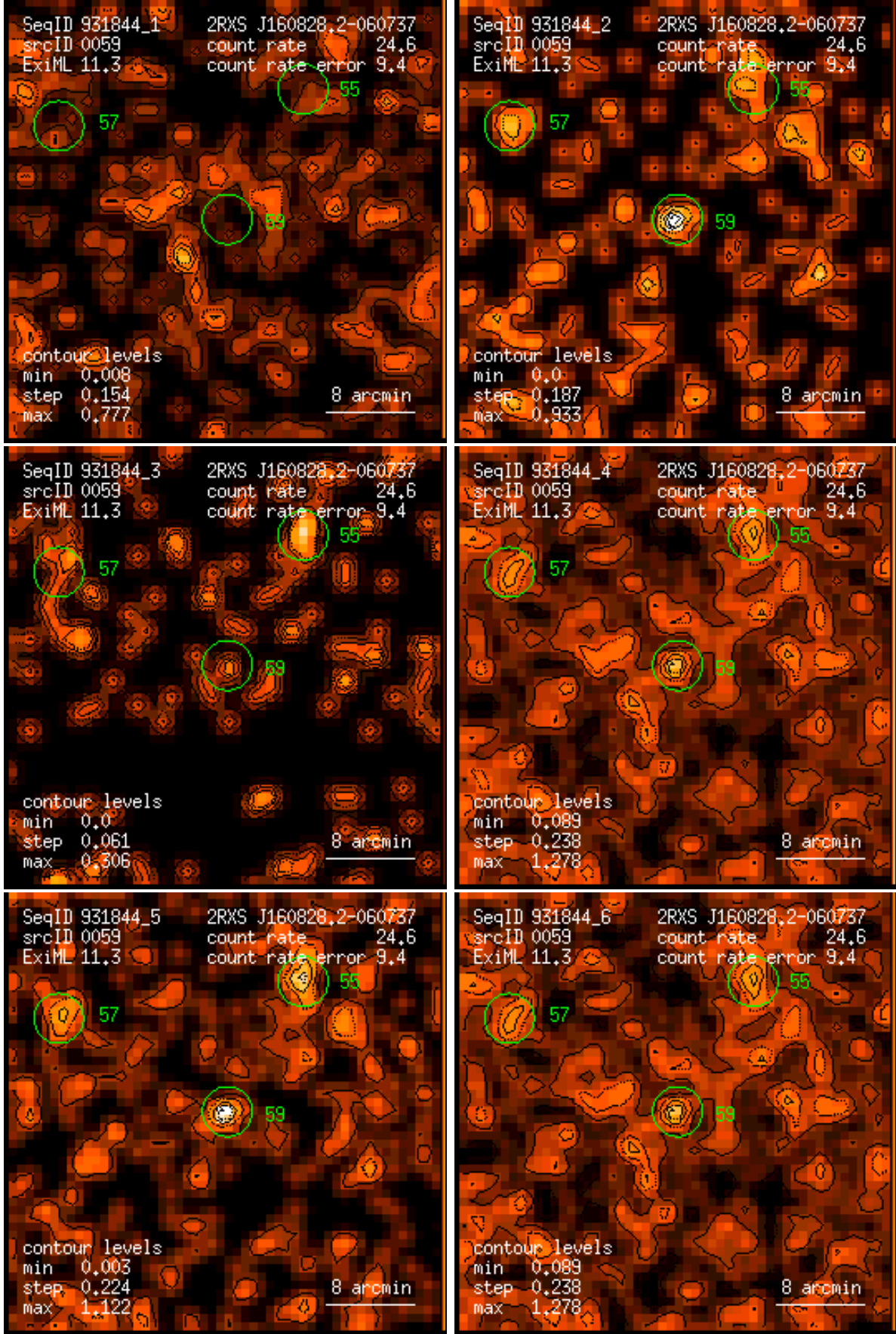
Figure 59: RASS 931844: detection 0059: band rate images, Gaussian filter: (1) PSPC channels 11 – 41, (2) 52 – 90, (3) 91 – 201, (4) 11 – 235, (5) 52 – 201, (6) 11 – 201. Broad band rates in counts/ks. Band rate contour levels in counts/ks/arcmin 2 .
