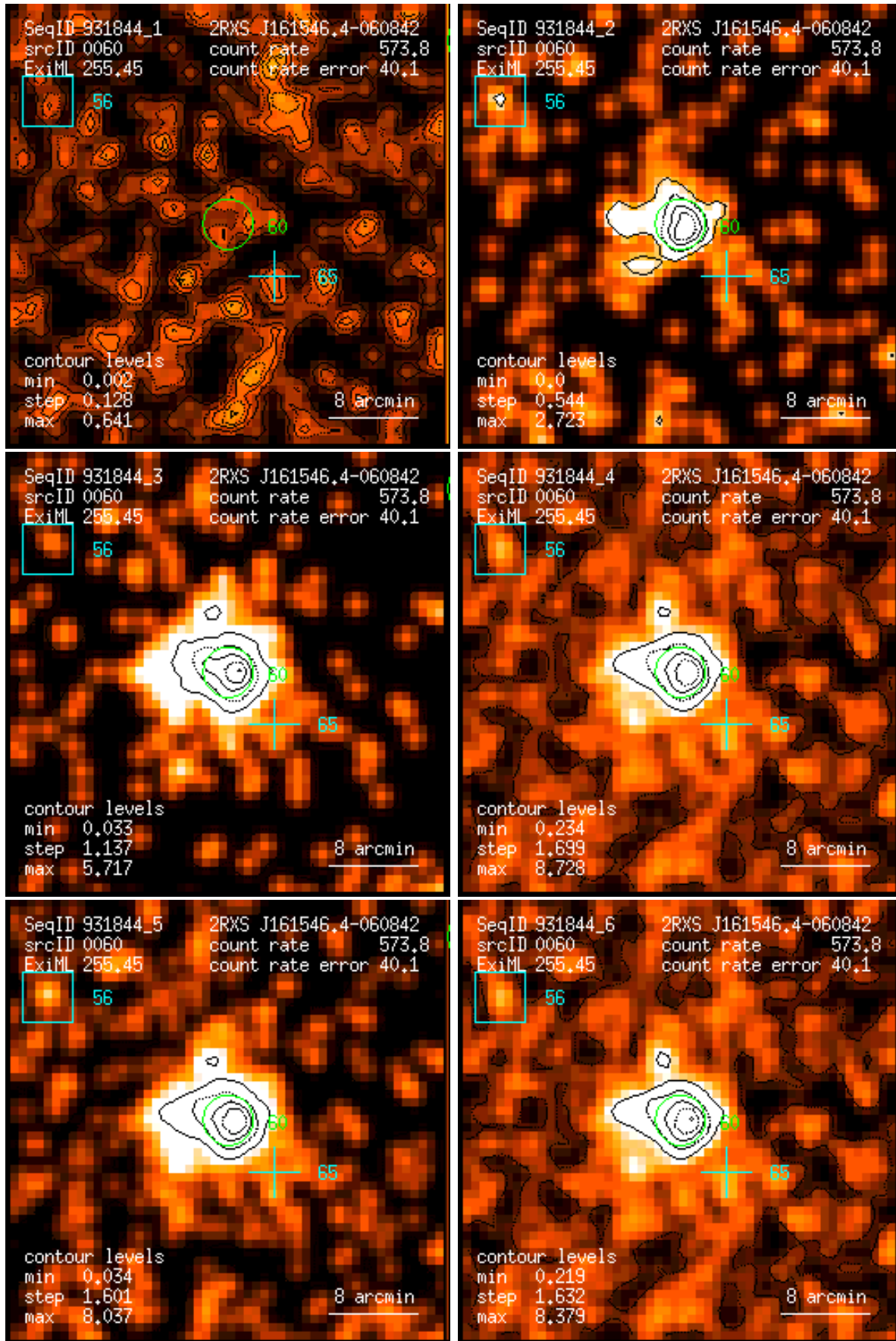
Figure 60: RASS 931844: detection 0060: band rate images, Gaussian filter: (1) PSPC channels 11 – 41, (2) 52 – 90, (3) 91 – 201, (4) 11 – 235, (5) 52 – 201, (6) 11 – 201. Broad band rates in counts/ks. Band rate contour levels in counts/ks/arcmin 2 .
