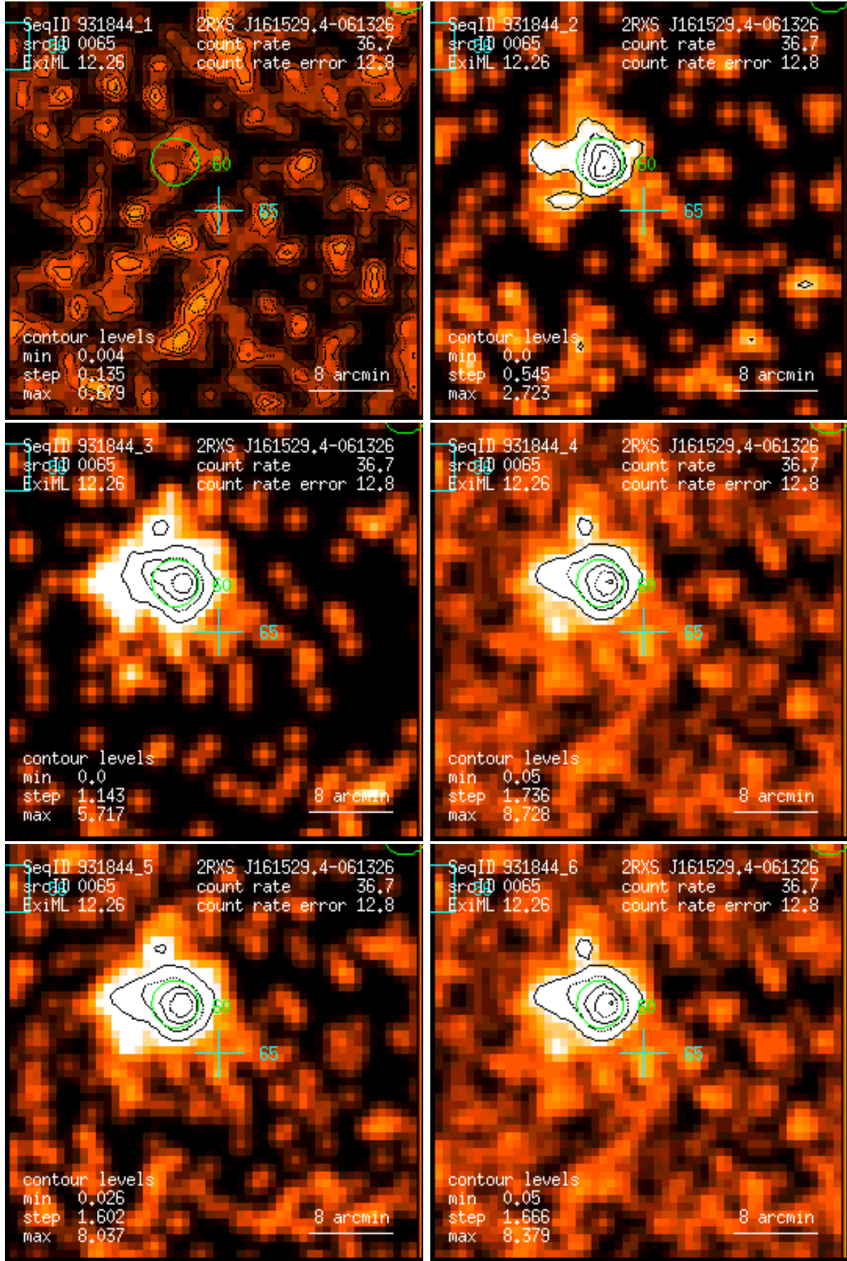
Figure 65: RASS 931844: detection 0065: band rate images, Gaussian filter: (1) PSPC channels 11 – 41, (2) 52 – 90, (3) 91 – 201, (4) 11 – 235, (5) 52 – 201, (6) 11 – 201. Broad band rates in counts/ks. Band rate contour levels in counts/ks/arcmin 2 .
