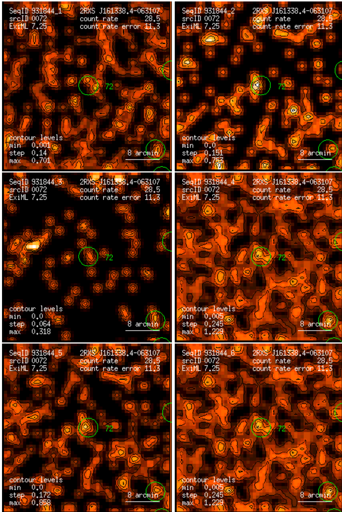
Figure 72: RASS 931844: detection 0072: band rate images, Gaussian filter: (1) PSPC channels 11 – 41, (2) 52 – 90, (3) 91 – 201, (4) 11 – 235, (5) 52 – 201, (6) 11 – 201. Broad band rates in counts/ks. Band rate contour levels in counts/ks/arcmin 2 .
