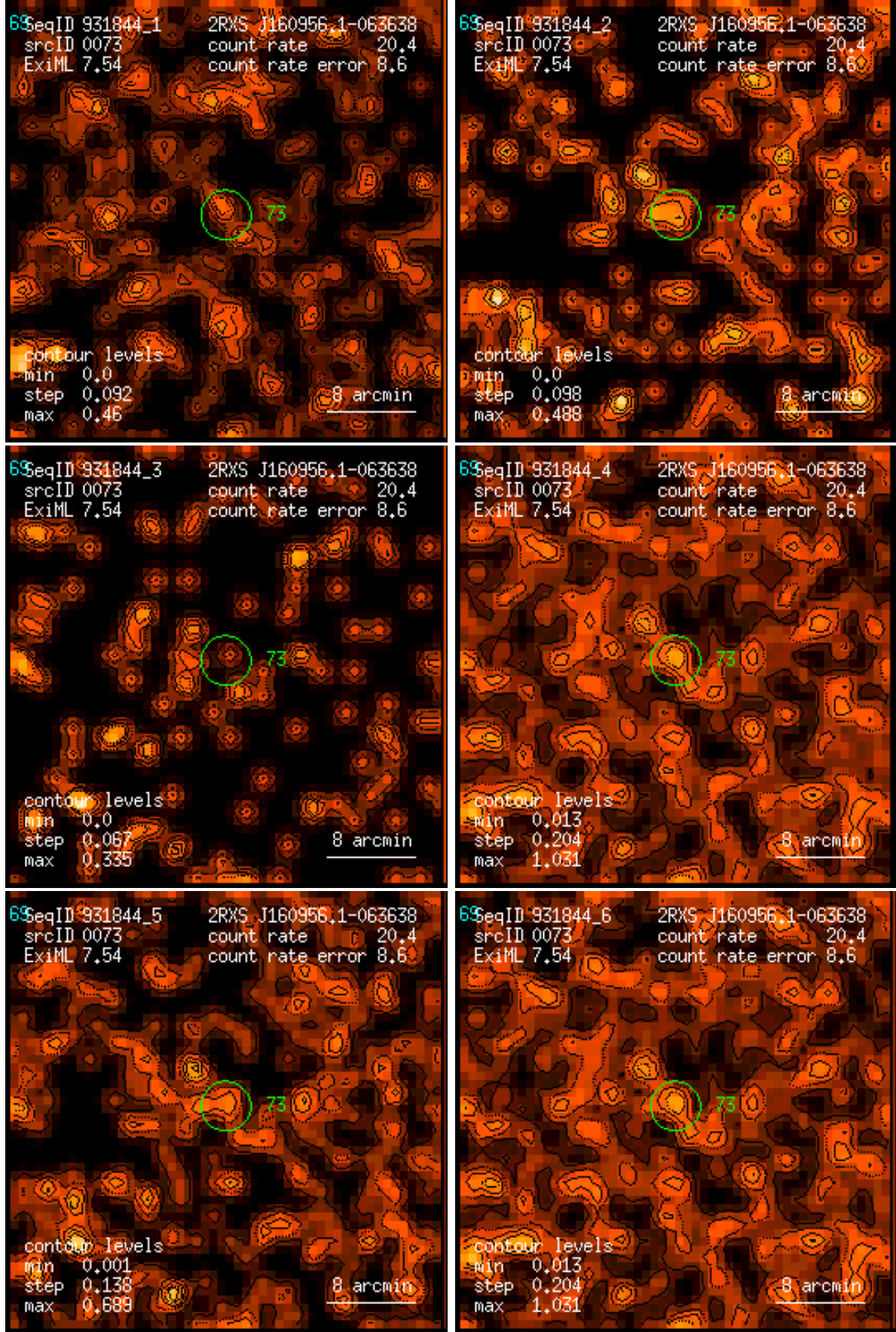
Figure 73: RASS 931844: detection 0073: band rate images, Gaussian filter: (1) PSPC channels 11 – 41, (2) 52 – 90, (3) 91 – 201, (4) 11 – 235, (5) 52 – 201, (6) 11 – 201. Broad band rates in counts/ks. Band rate contour levels in counts/ks/arcmin 2 .
