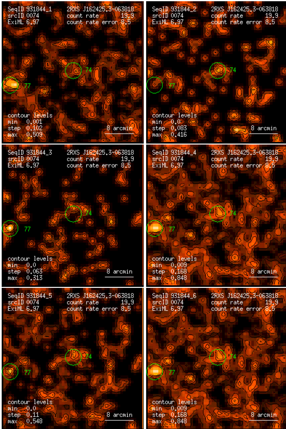
Figure 74: RASS 931844: detection 0074: band rate images, Gaussian filter: (1) PSPC channels 11 – 41, (2) 52 – 90, (3) 91 – 201, (4) 11 – 235, (5) 52 – 201, (6) 11 – 201. Broad band rates in counts/ks. Band rate contour levels in counts/ks/arcmin 2 .
