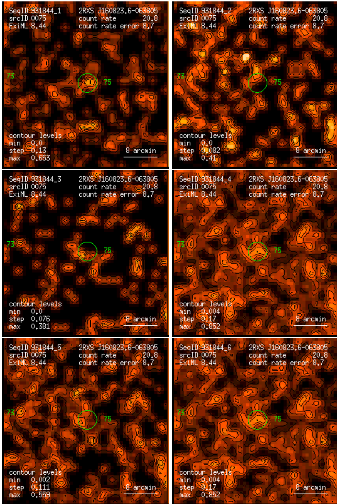
Figure 75: RASS 931844: detection 0075: band rate images, Gaussian filter: (1) PSPC channels 11 – 41, (2) 52 – 90, (3) 91 – 201, (4) 11 – 235, (5) 52 – 201, (6) 11 – 201. Broad band rates in counts/ks. Band rate contour levels in counts/ks/arcmin 2 .
