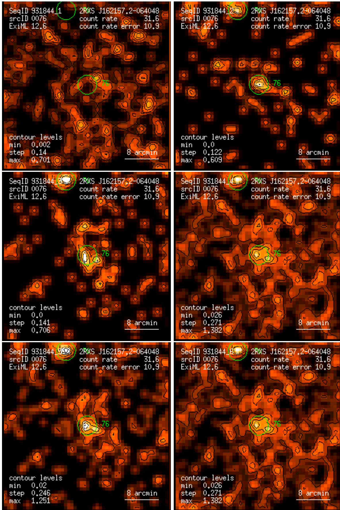
Figure 76: RASS 931844: detection 0076: band rate images, Gaussian filter: (1) PSPC channels 11 – 41, (2) 52 – 90, (3) 91 – 201, (4) 11 – 235, (5) 52 – 201, (6) 11 – 201. Broad band rates in counts/ks. Band rate contour levels in counts/ks/arcmin 2 .
