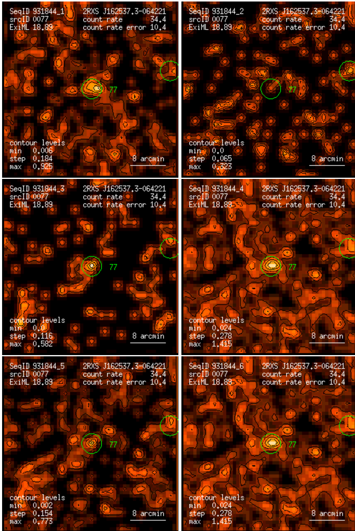
Figure 77: RASS 931844: detection 0077: band rate images, Gaussian filter: (1) PSPC channels 11 – 41, (2) 52 – 90, (3) 91 – 201, (4) 11 – 235, (5) 52 – 201, (6) 11 – 201. Broad band rates in counts/ks. Band rate contour levels in counts/ks/arcmin 2 .
