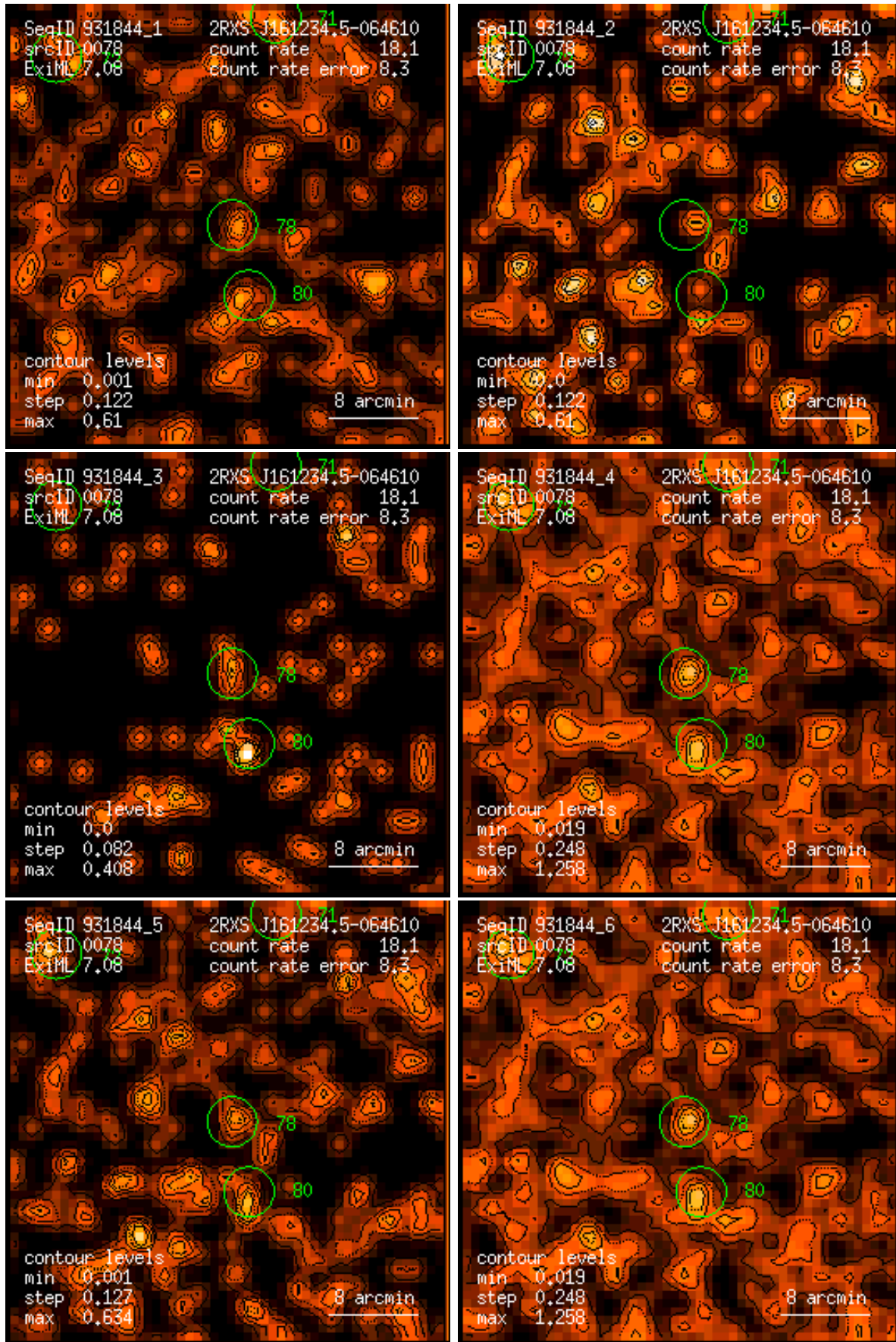
Figure 78: RASS 931844: detection 0078: band rate images, Gaussian filter: (1) PSPC channels 11 – 41, (2) 52 – 90, (3) 91 – 201, (4) 11 – 235, (5) 52 – 201, (6) 11 – 201. Broad band rates in counts/ks. Band rate contour levels in counts/ks/arcmin 2 .
