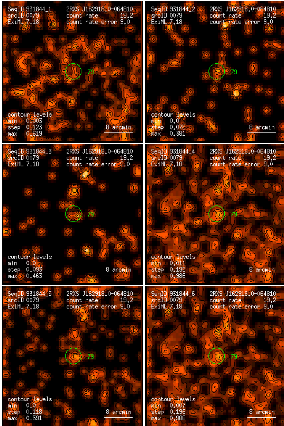
Figure 79: RASS 931844: detection 0079: band rate images, Gaussian filter: (1) PSPC channels 11 – 41, (2) 52 – 90, (3) 91 – 201, (4) 11 – 235, (5) 52 – 201, (6) 11 – 201. Broad band rates in counts/ks. Band rate contour levels in counts/ks/arcmin 2 .
