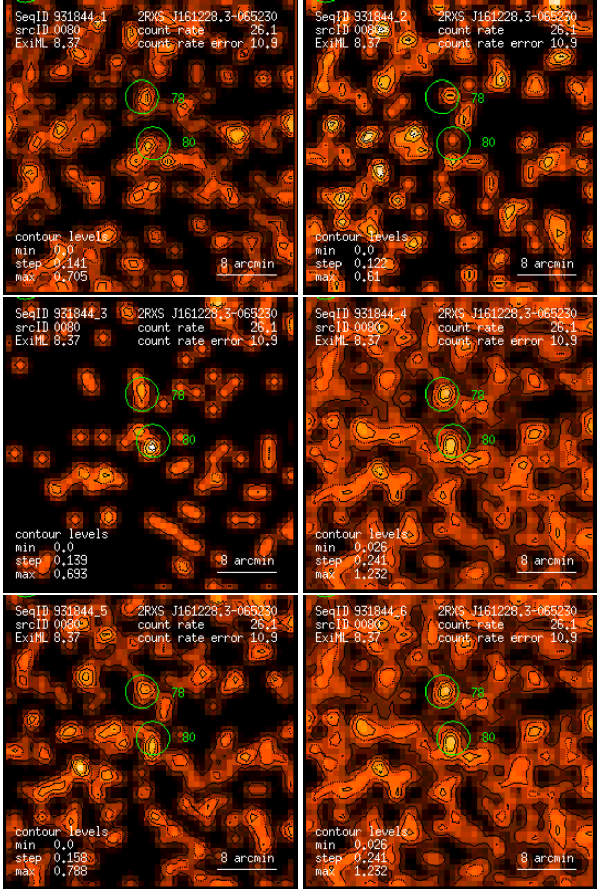
Figure 80: RASS 931844: detection 0080: band rate images, Gaussian filter: (1) PSPC channels 11 – 41, (2) 52 – 90, (3) 91 – 201, (4) 11 – 235, (5) 52 – 201, (6) 11 – 201. Broad band rates in counts/ks. Band rate contour levels in counts/ks/arcmin 2 .
