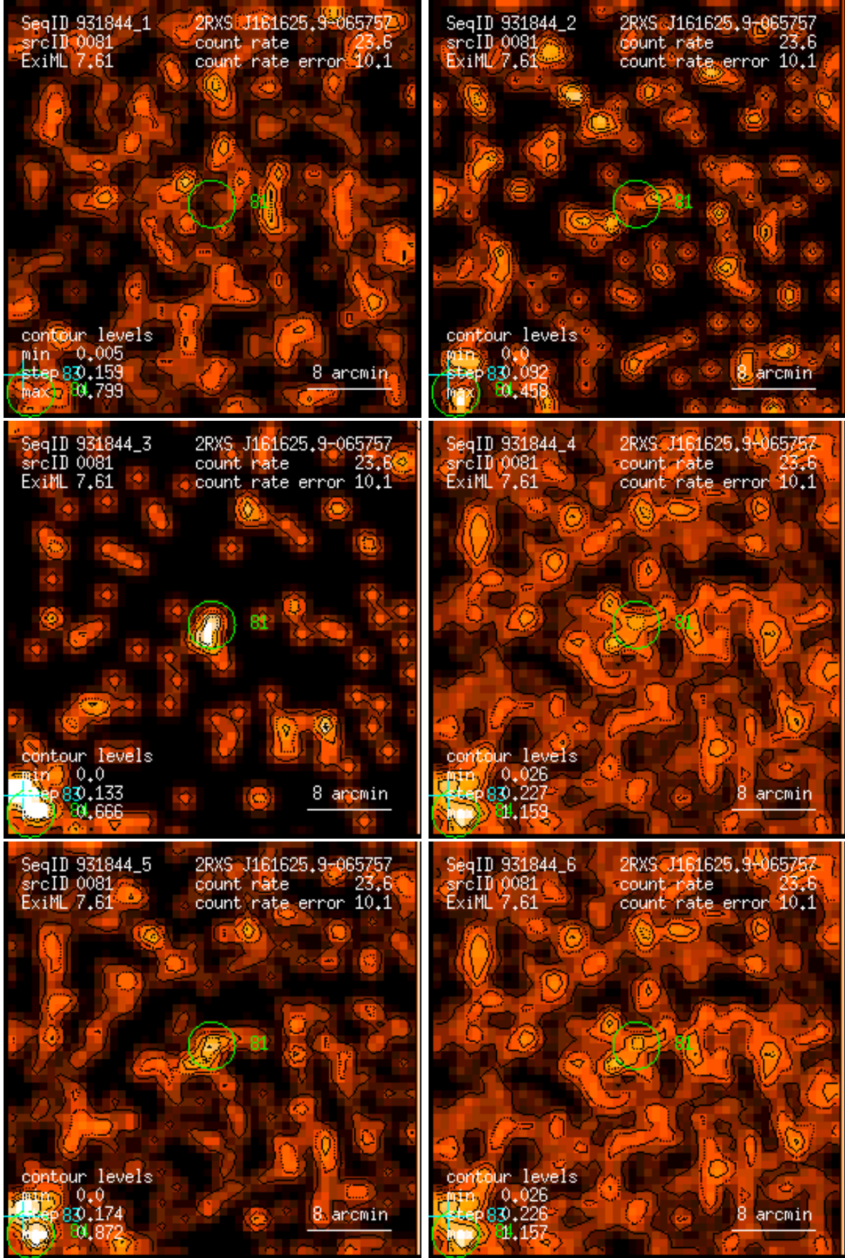
Figure 81: RASS 931844: detection 0081: band rate images, Gaussian filter: (1) PSPC channels 11 – 41, (2) 52 – 90, (3) 91 – 201, (4) 11 – 235, (5) 52 – 201, (6) 11 – 201. Broad band rates in counts/ks. Band rate contour levels in counts/ks/arcmin 2 .
