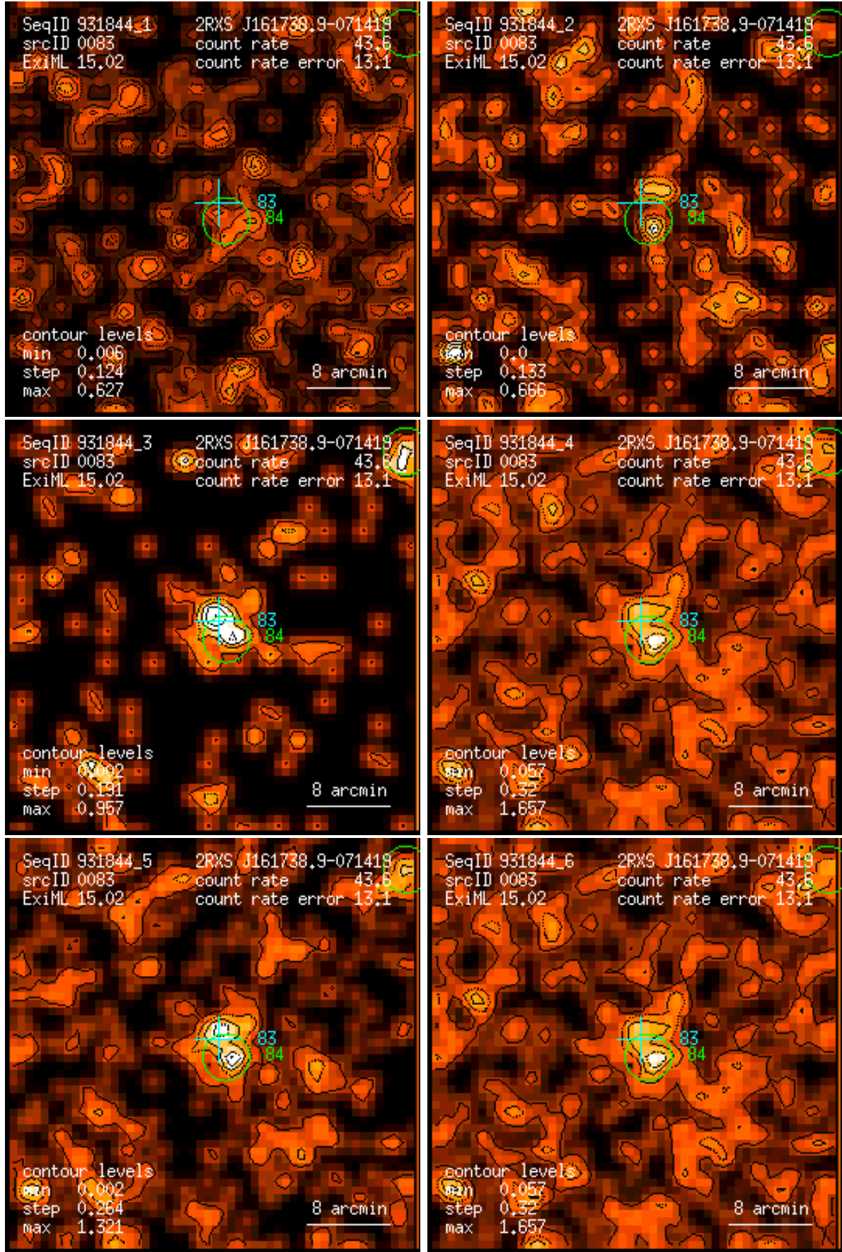
Figure 83: RASS 931844: detection 0083: band rate images, Gaussian filter: (1) PSPC channels 11 – 41, (2) 52 – 90, (3) 91 – 201, (4) 11 – 235, (5) 52 – 201, (6) 11 – 201. Broad band rates in counts/ks. Band rate contour levels in counts/ks/arcmin 2 .
