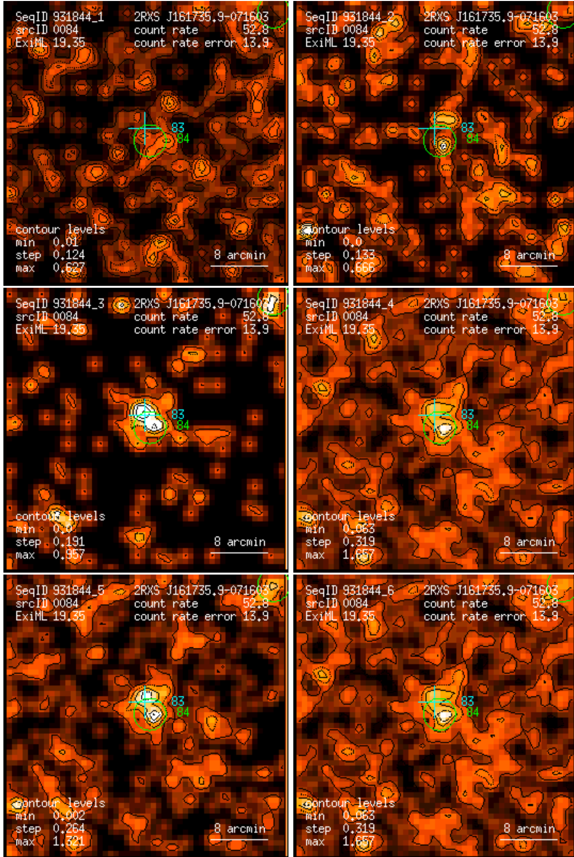
Figure 84: RASS 931844: detection 0084: band rate images, Gaussian filter: (1) PSPC channels 11 – 41, (2) 52 – 90, (3) 91 – 201, (4) 11 – 235, (5) 52 – 201, (6) 11 – 201. Broad band rates in counts/ks. Band rate contour levels in counts/ks/arcmin 2 .
